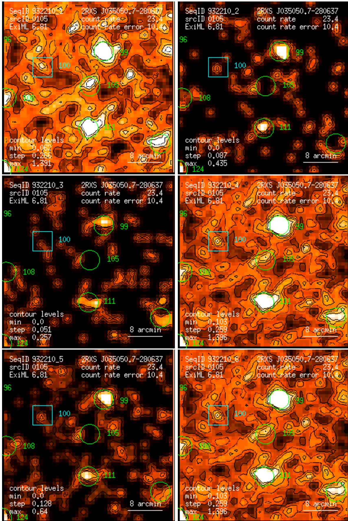
Figure 105: RASS 932210: detection 0105: band rate images, Gaussian filter: (1) PSPC channels 11 – 41, (2) 52 – 90, (3) 91 – 201, (4) 11 – 235, (5) 52 – 201, (6) 11 – 201. Broad band rates in counts/ks. Band rate contour levels in counts/ks/arcmin 2 .
