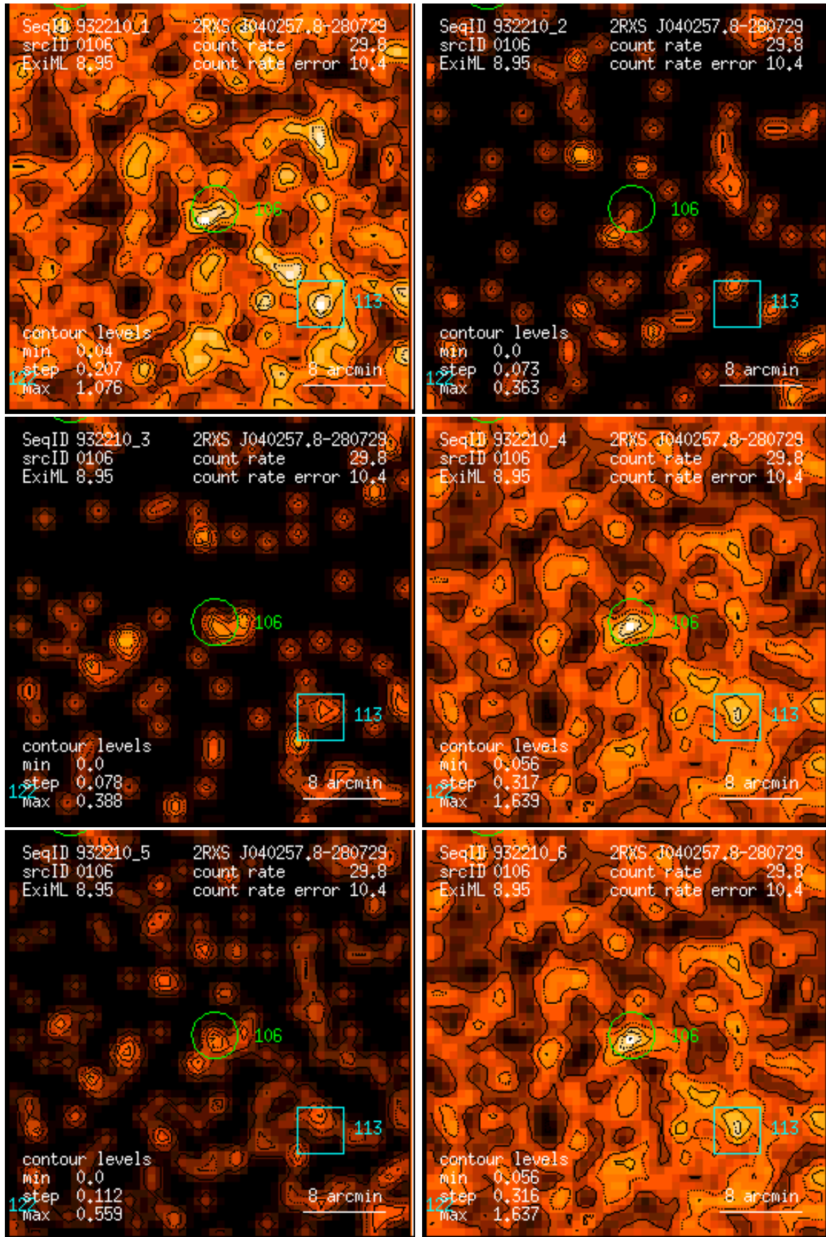
Figure 106: RASS 932210: detection 0106: band rate images, Gaussian filter: (1) PSPC channels 11 – 41, (2) 52 – 90, (3) 91 – 201, (4) 11 – 235, (5) 52 – 201, (6) 11 – 201. Broad band rates in counts/ks. Band rate contour levels in counts/ks/arcmin 2 .
