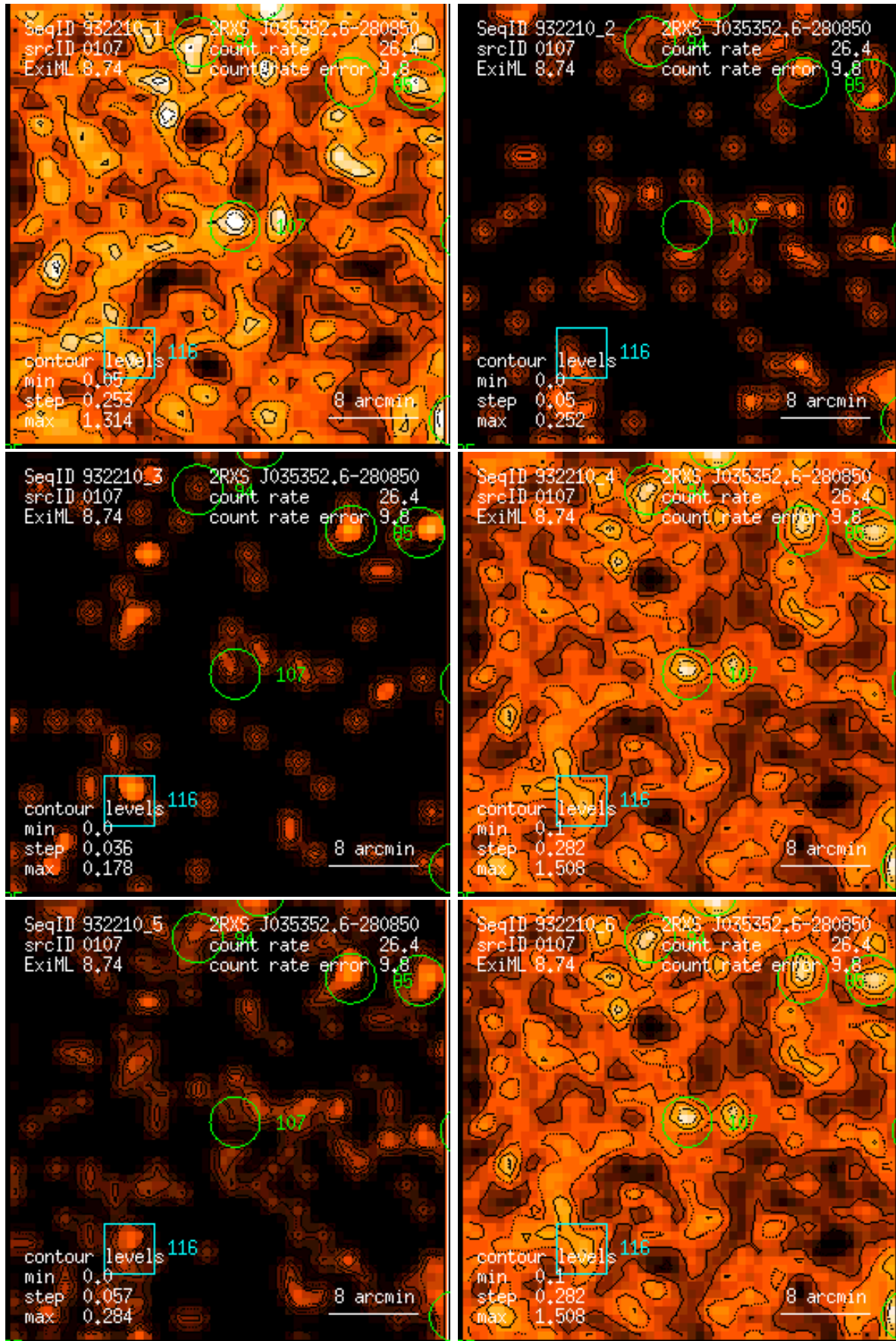
Figure 107: RASS 932210: detection 0107: band rate images, Gaussian filter: (1) PSPC channels 11 – 41, (2) 52 – 90, (3) 91 – 201, (4) 11 – 235, (5) 52 – 201, (6) 11 – 201. Broad band rates in counts/ks. Band rate contour levels in counts/ks/arcmin 2 .
