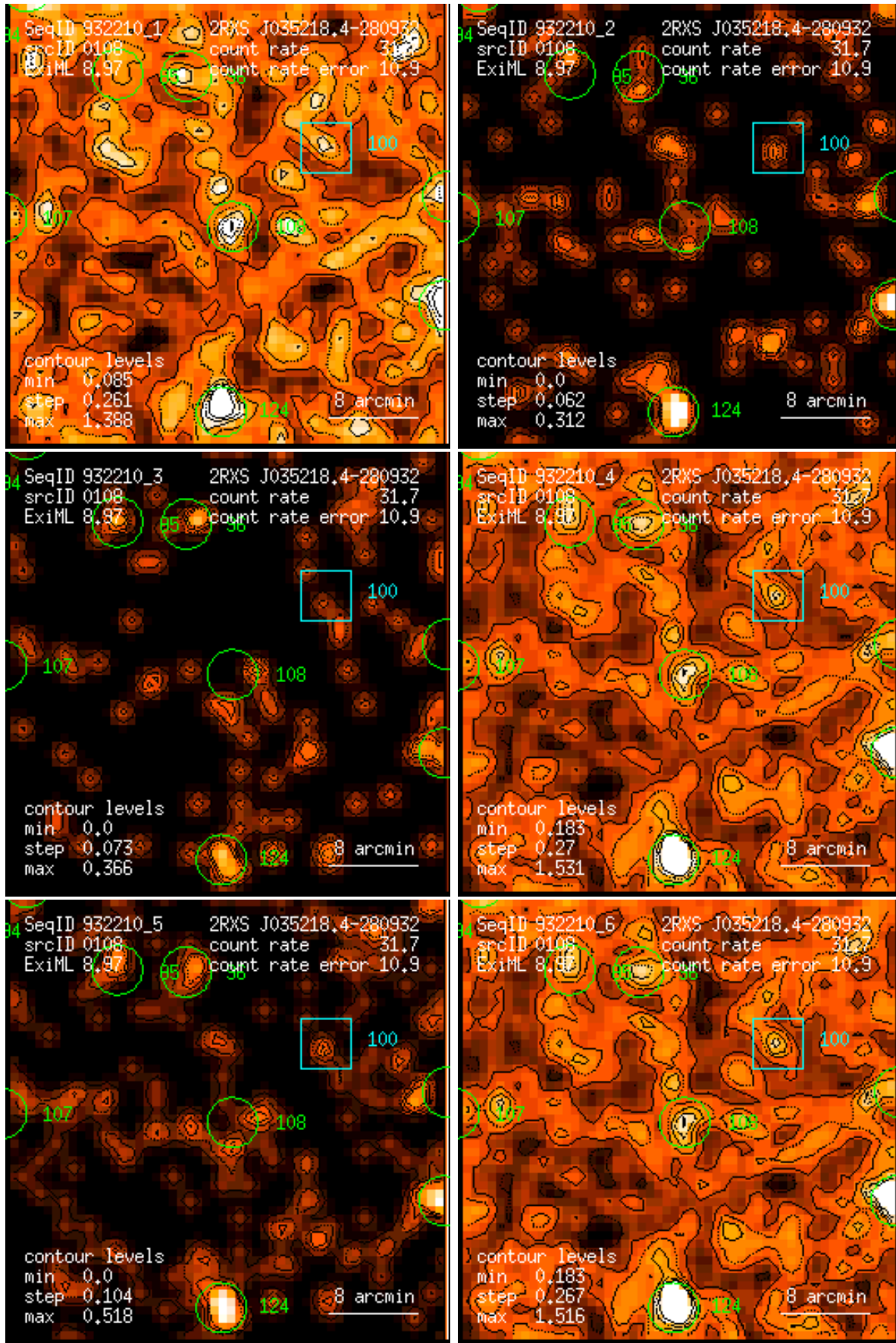
Figure 108: RASS 932210: detection 0108: band rate images, Gaussian filter: (1) PSPC channels 11 – 41, (2) 52 – 90, (3) 91 – 201, (4) 11 – 235, (5) 52 – 201, (6) 11 – 201. Broad band rates in counts/ks. Band rate contour levels in counts/ks/arcmin 2 .
