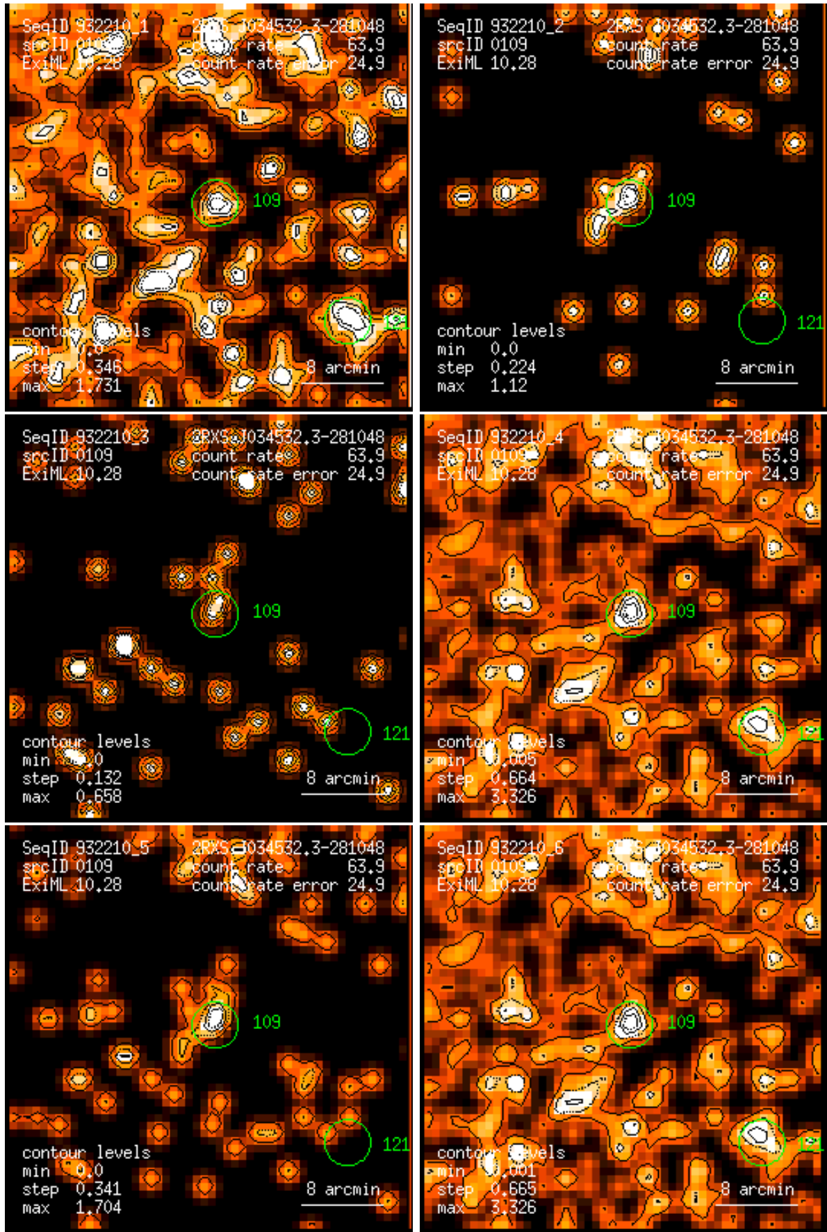
Figure 109: RASS 932210: detection 0109: band rate images, Gaussian filter: (1) PSPC channels 11 – 41, (2) 52 – 90, (3) 91 – 201, (4) 11 – 235, (5) 52 – 201, (6) 11 – 201. Broad band rates in counts/ks. Band rate contour levels in counts/ks/arcmin 2 .
