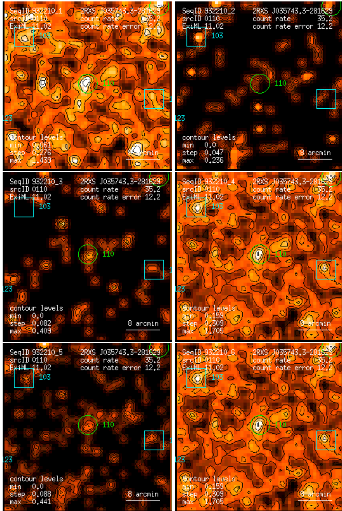
Figure 110: RASS 932210: detection 0110: band rate images, Gaussian filter: (1) PSPC channels 11 – 41, (2) 52 – 90, (3) 91 – 201, (4) 11 – 235, (5) 52 – 201, (6) 11 – 201. Broad band rates in counts/ks. Band rate contour levels in counts/ks/arcmin 2 .
