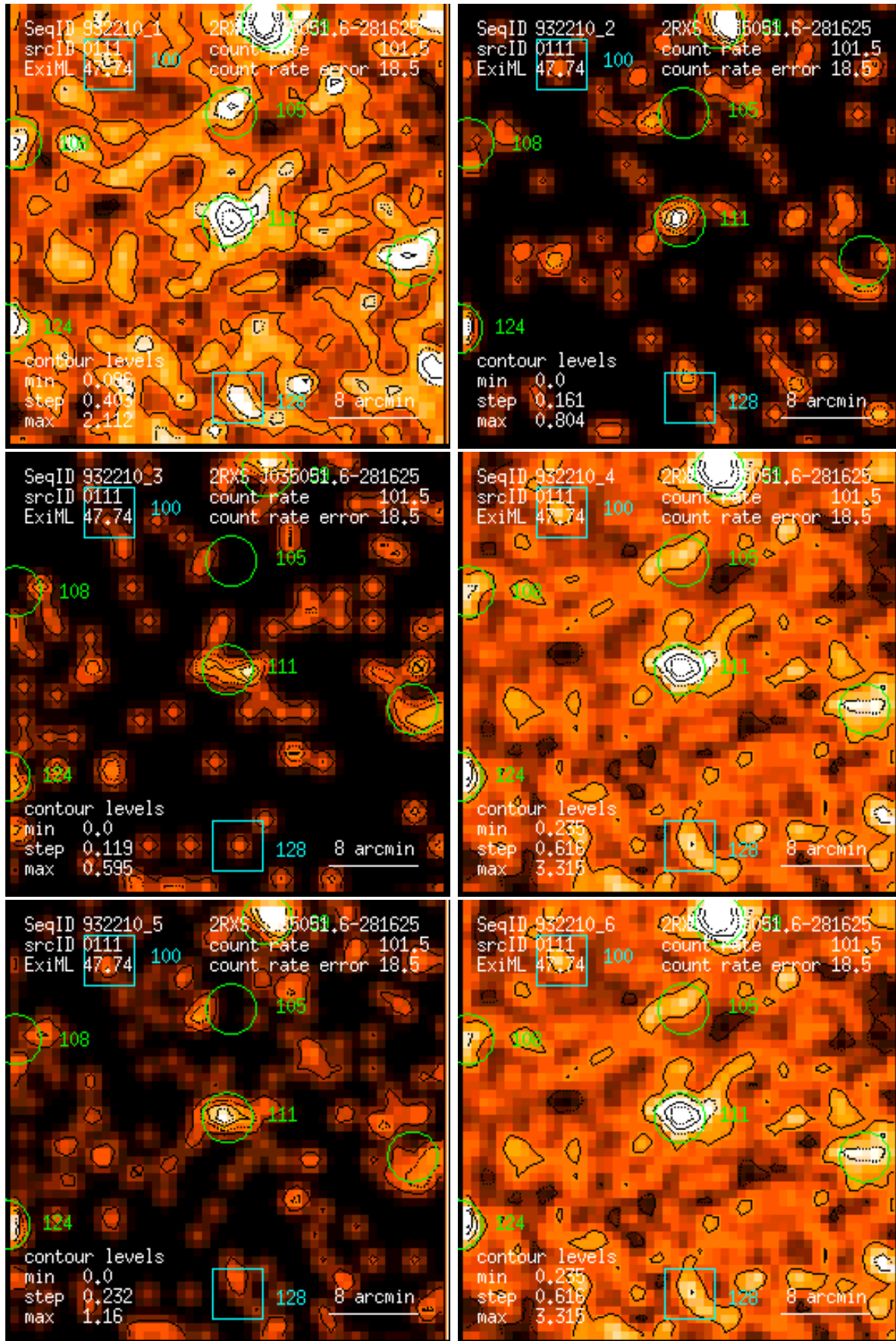
Figure 111: RASS 932210: detection 0111: band rate images, Gaussian filter: (1) PSPC channels 11 – 41, (2) 52 – 90, (3) 91 – 201, (4) 11 – 235, (5) 52 – 201, (6) 11 – 201. Broad band rates in counts/ks. Band rate contour levels in counts/ks/arcmin 2 .
