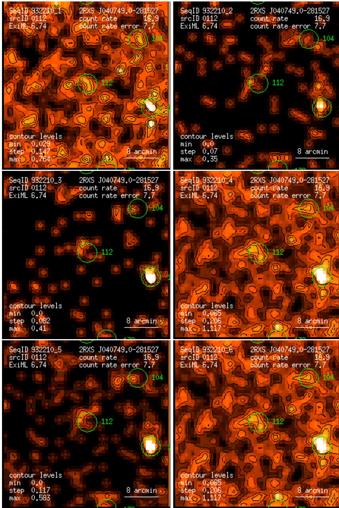
Figure 112: RASS 932210: detection 0112: band rate images, Gaussian filter: (1) PSPC channels 11 – 41, (2) 52 – 90, (3) 91 – 201, (4) 11 – 235, (5) 52 – 201, (6) 11 – 201. Broad band rates in counts/ks. Band rate contour levels in counts/ks/arcmin 2 .
