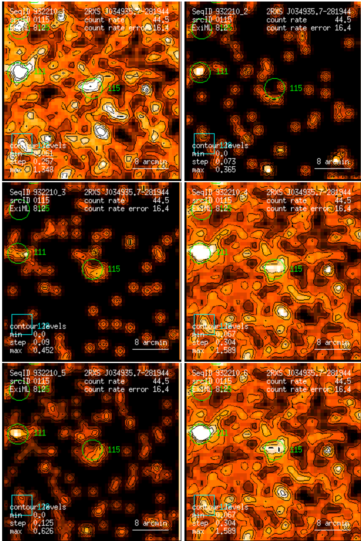
Figure 115: RASS 932210: detection 0115: band rate images, Gaussian filter: (1) PSPC channels 11 – 41, (2) 52 – 90, (3) 91 – 201, (4) 11 – 235, (5) 52 – 201, (6) 11 – 201. Broad band rates in counts/ks. Band rate contour levels in counts/ks/arcmin 2 .
