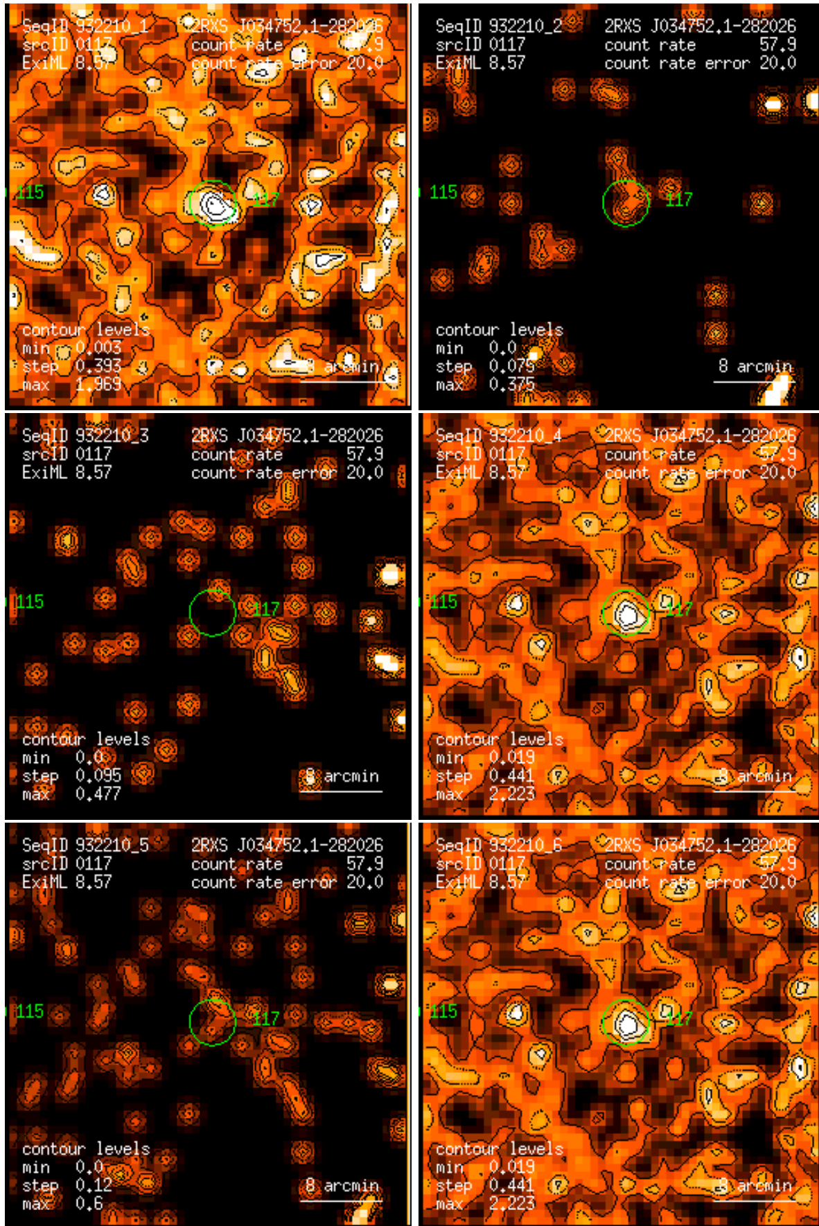
Figure 117: RASS 932210: detection 0117: band rate images, Gaussian filter: (1) PSPC channels 11 – 41, (2) 52 – 90, (3) 91 – 201, (4) 11 – 235, (5) 52 – 201, (6) 11 – 201. Broad band rates in counts/ks. Band rate contour levels in counts/ks/arcmin 2 .
