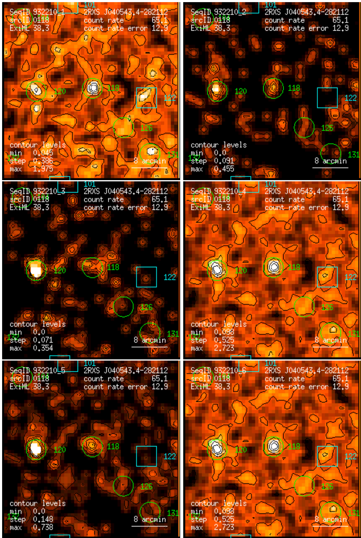
Figure 118: RASS 932210: detection 0118: band rate images, Gaussian filter: (1) PSPC channels 11 – 41, (2) 52 – 90, (3) 91 – 201, (4) 11 – 235, (5) 52 – 201, (6) 11 – 201. Broad band rates in counts/ks. Band rate contour levels in counts/ks/arcmin 2 .
