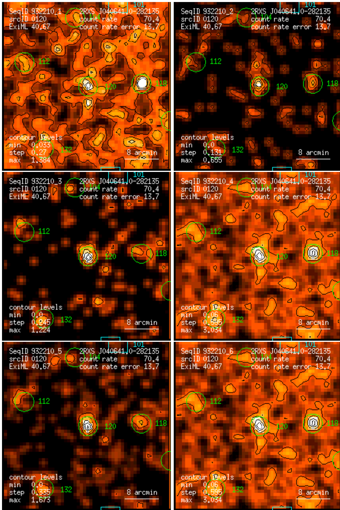
Figure 120: RASS 932210: detection 0120: band rate images, Gaussian filter: (1) PSPC channels 11 – 41, (2) 52 – 90, (3) 91 – 201, (4) 11 – 235, (5) 52 – 201, (6) 11 – 201. Broad band rates in counts/ks. Band rate contour levels in counts/ks/arcmin 2 .
