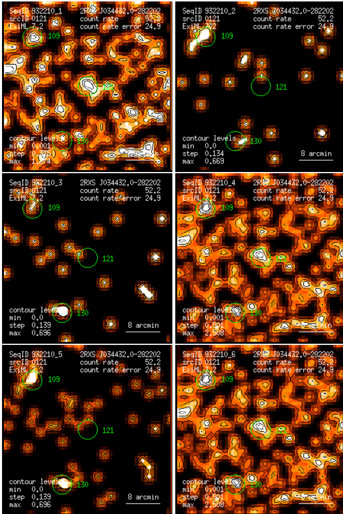
Figure 121: RASS 932210: detection 0121: band rate images, Gaussian filter: (1) PSPC channels 11 – 41, (2) 52 – 90, (3) 91 – 201, (4) 11 – 235, (5) 52 – 201, (6) 11 – 201. Broad band rates in counts/ks. Band rate contour levels in counts/ks/arcmin 2 .
