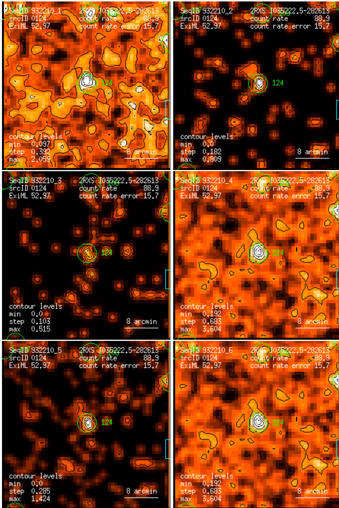
Figure 124: RASS 932210: detection 0124: band rate images, Gaussian filter: (1) PSPC channels 11 – 41, (2) 52 – 90, (3) 91 – 201, (4) 11 – 235, (5) 52 – 201, (6) 11 – 201. Broad band rates in counts/ks. Band rate contour levels in counts/ks/arcmin 2 .
