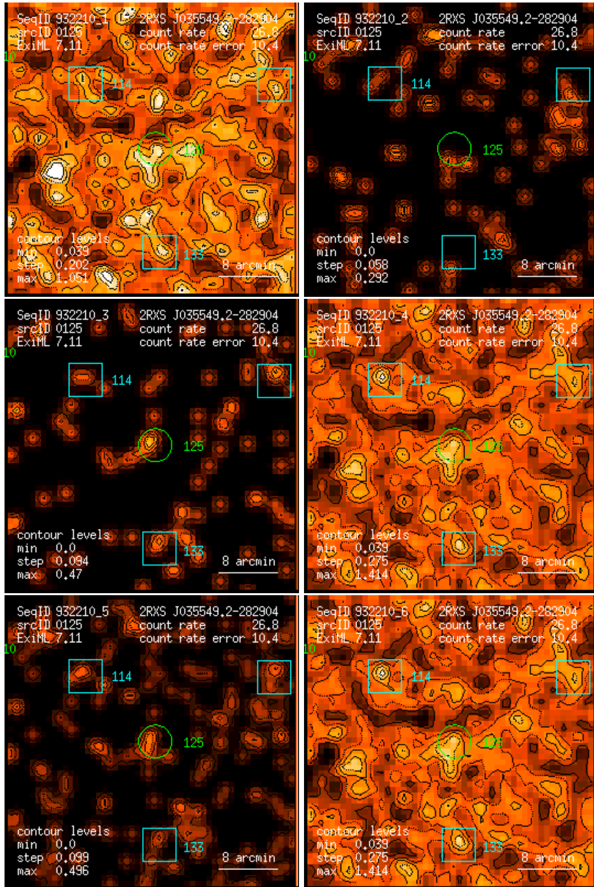
Figure 125: RASS 932210: detection 0125: band rate images, Gaussian filter: (1) PSPC channels 11 – 41, (2) 52 – 90, (3) 91 – 201, (4) 11 – 235, (5) 52 – 201, (6) 11 – 201. Broad band rates in counts/ks. Band rate contour levels in counts/ks/arcmin 2 .
