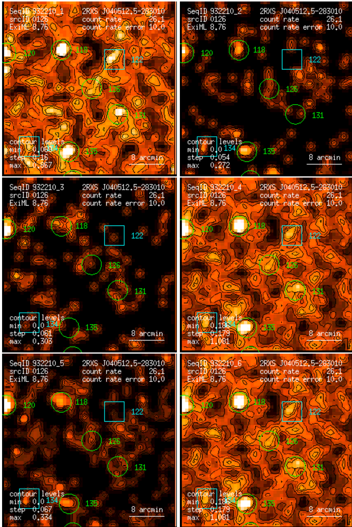
Figure 126: RASS 932210: detection 0126: band rate images, Gaussian filter: (1) PSPC channels 11 – 41, (2) 52 – 90, (3) 91 – 201, (4) 11 – 235, (5) 52 – 201, (6) 11 – 201. Broad band rates in counts/ks. Band rate contour levels in counts/ks/arcmin 2 .
