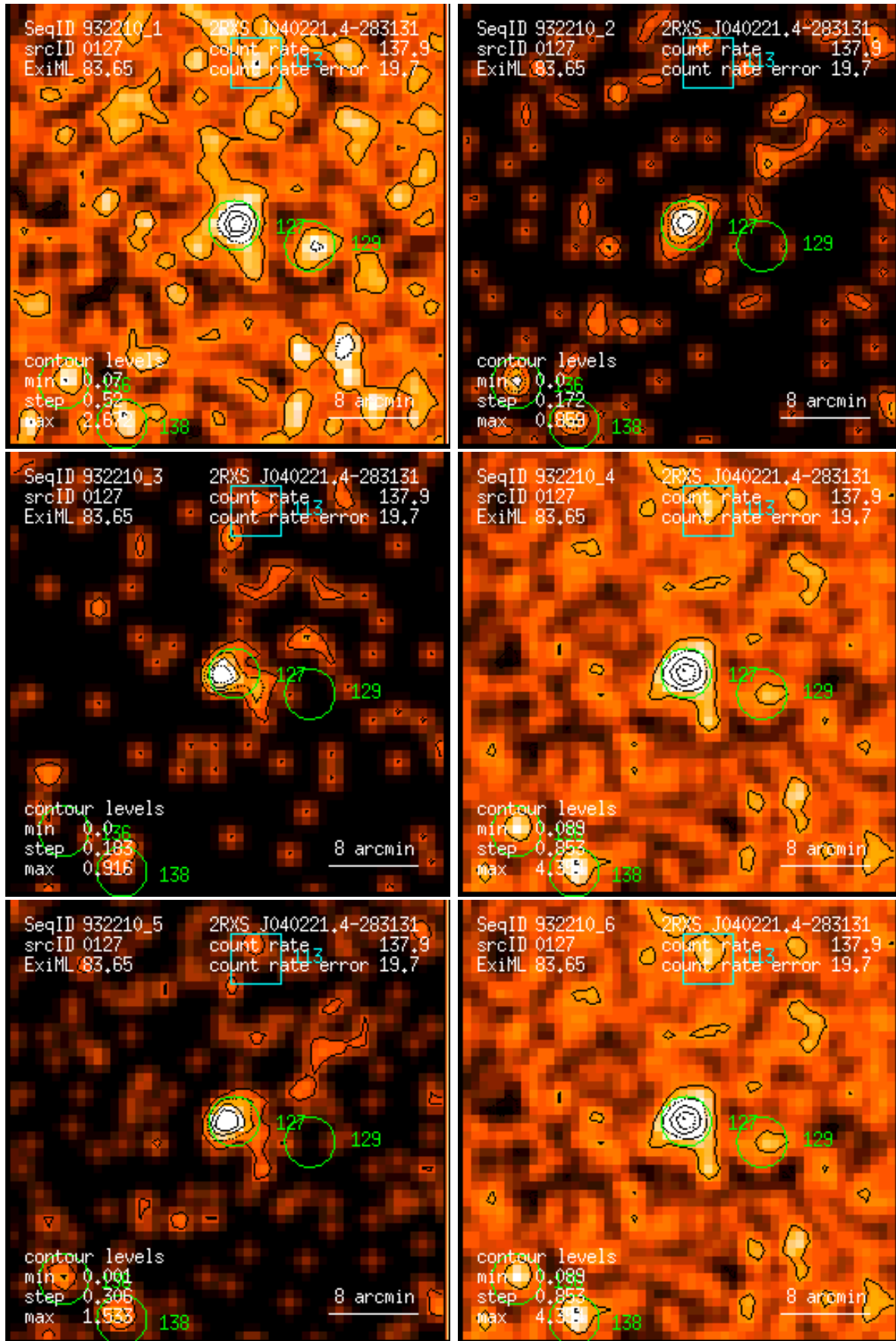
Figure 127: RASS 932210: detection 0127: band rate images, Gaussian filter: (1) PSPC channels 11 – 41, (2) 52 – 90, (3) 91 – 201, (4) 11 – 235, (5) 52 – 201, (6) 11 – 201. Broad band rates in counts/ks. Band rate contour levels in counts/ks/arcmin 2 .
