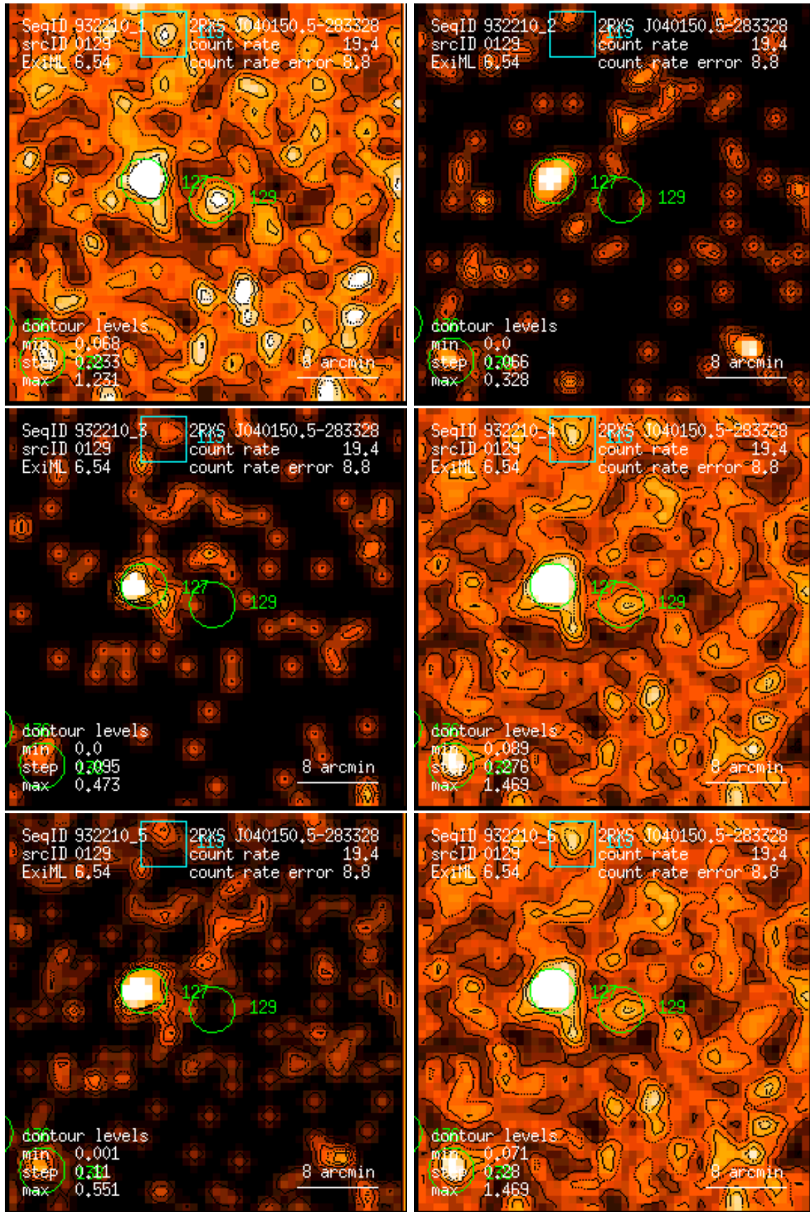
Figure 129: RASS 932210: detection 0129: band rate images, Gaussian filter: (1) PSPC channels 11 – 41, (2) 52 – 90, (3) 91 – 201, (4) 11 – 235, (5) 52 – 201, (6) 11 – 201. Broad band rates in counts/ks. Band rate contour levels in counts/ks/arcmin 2 .
