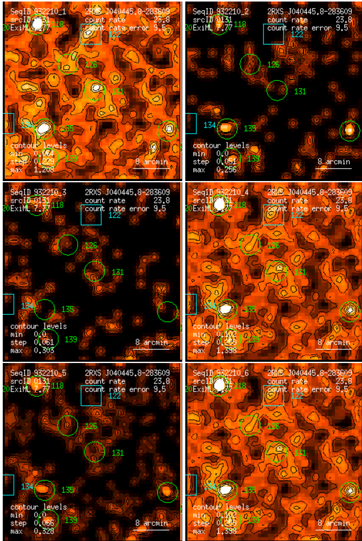
Figure 131: RASS 932210: detection 0131: band rate images, Gaussian filter: (1) PSPC channels 11 – 41, (2) 52 – 90, (3) 91 – 201, (4) 11 – 235, (5) 52 – 201, (6) 11 – 201. Broad band rates in counts/ks. Band rate contour levels in counts/ks/arcmin 2 .
