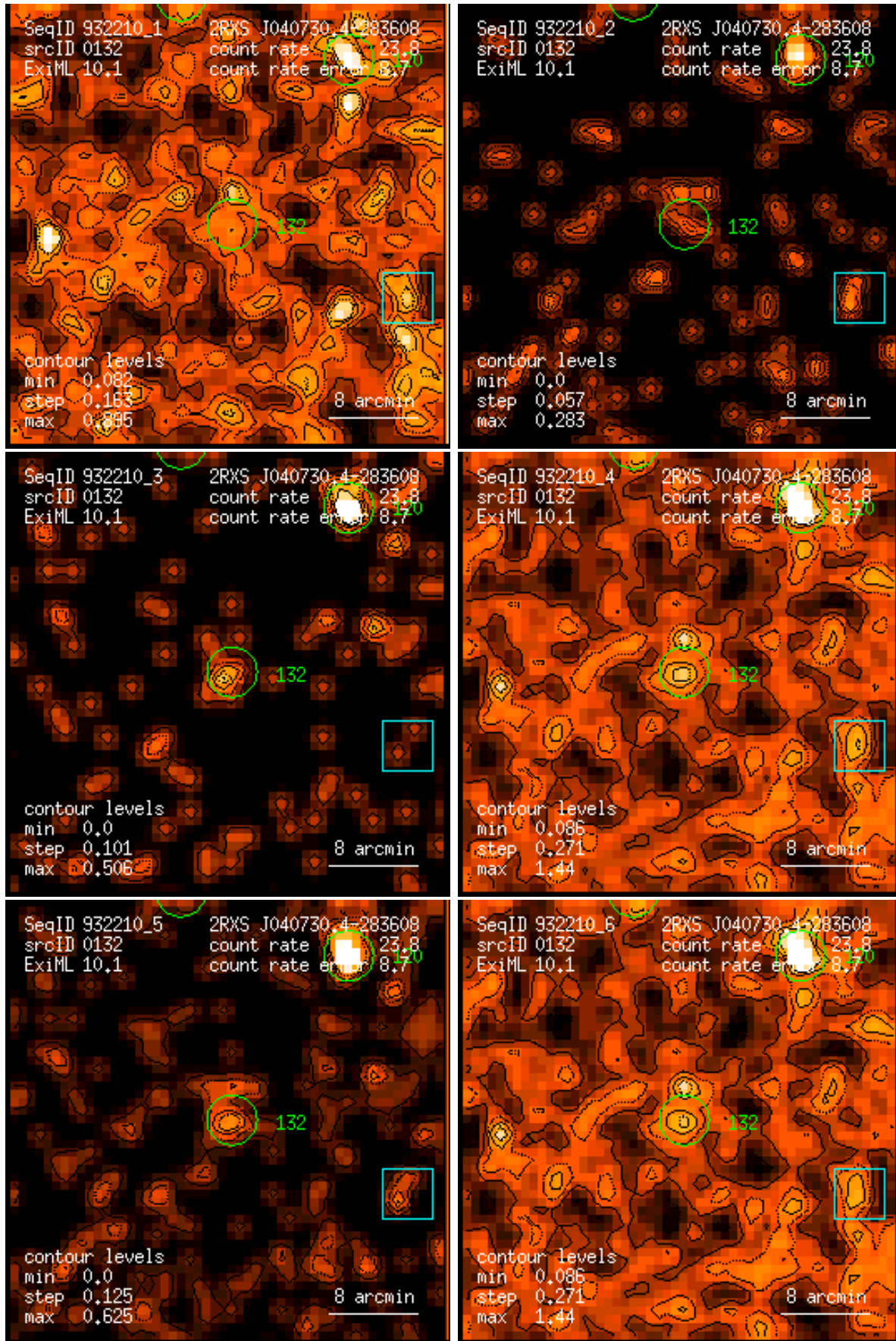
Figure 132: RASS 932210: detection 0132: band rate images, Gaussian filter: (1) PSPC channels 11 – 41, (2) 52 – 90, (3) 91 – 201, (4) 11 – 235, (5) 52 – 201, (6) 11 – 201. Broad band rates in counts/ks. Band rate contour levels in counts/ks/arcmin 2 .
