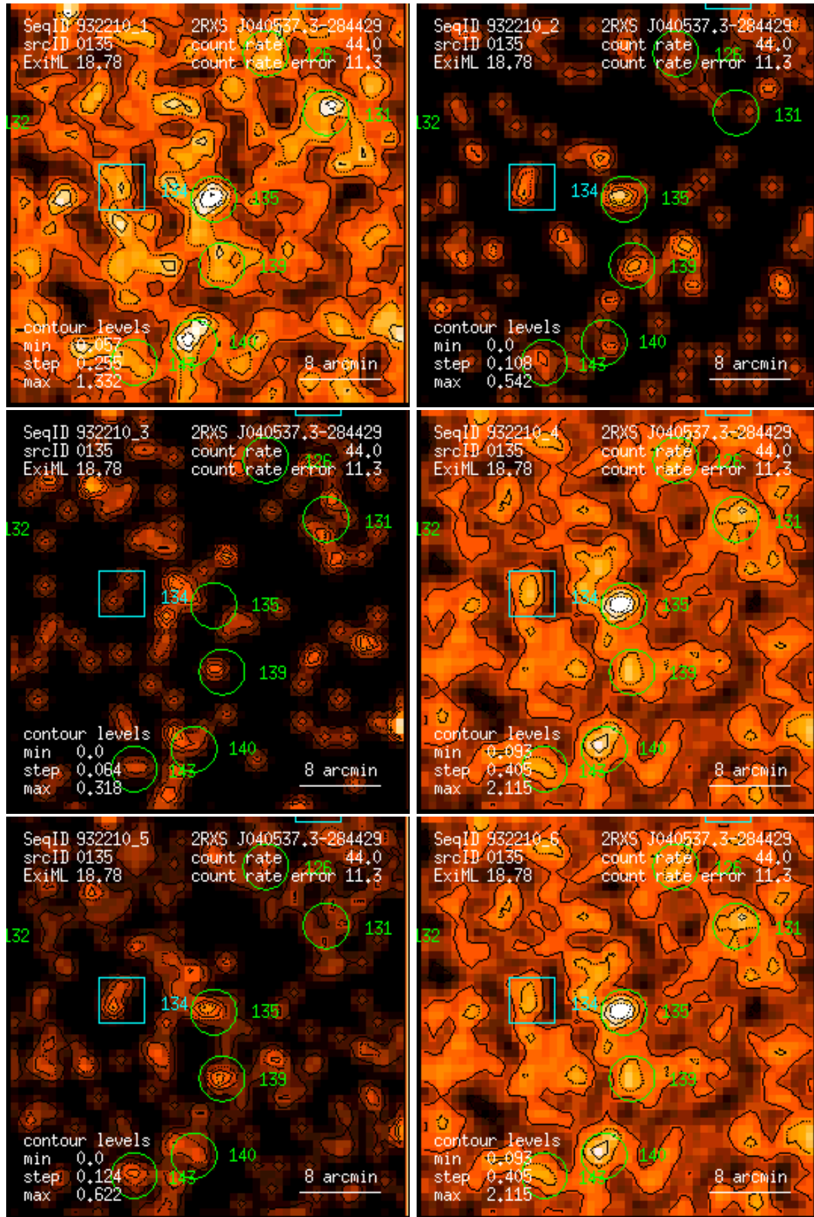
Figure 135: RASS 932210: detection 0135: band rate images, Gaussian filter: (1) PSPC channels 11 – 41, (2) 52 – 90, (3) 91 – 201, (4) 11 – 235, (5) 52 – 201, (6) 11 – 201. Broad band rates in counts/ks. Band rate contour levels in counts/ks/arcmin 2 .
