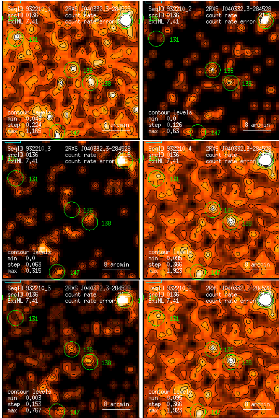
Figure 136: RASS 932210: detection 0136: band rate images, Gaussian filter: (1) PSPC channels 11 – 41, (2) 52 – 90, (3) 91 – 201, (4) 11 – 235, (5) 52 – 201, (6) 11 – 201. Broad band rates in counts/ks. Band rate contour levels in counts/ks/arcmin 2 .
