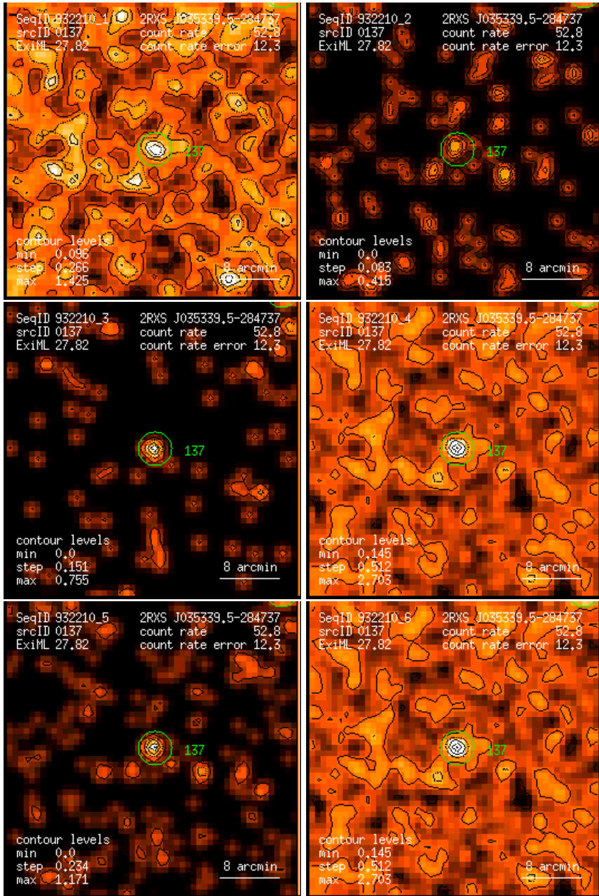
Figure 137: RASS 932210: detection 0137: band rate images, Gaussian filter: (1) PSPC channels 11 – 41, (2) 52 – 90, (3) 91 – 201, (4) 11 – 235, (5) 52 – 201, (6) 11 – 201. Broad band rates in counts/ks. Band rate contour levels in counts/ks/arcmin 2 .
