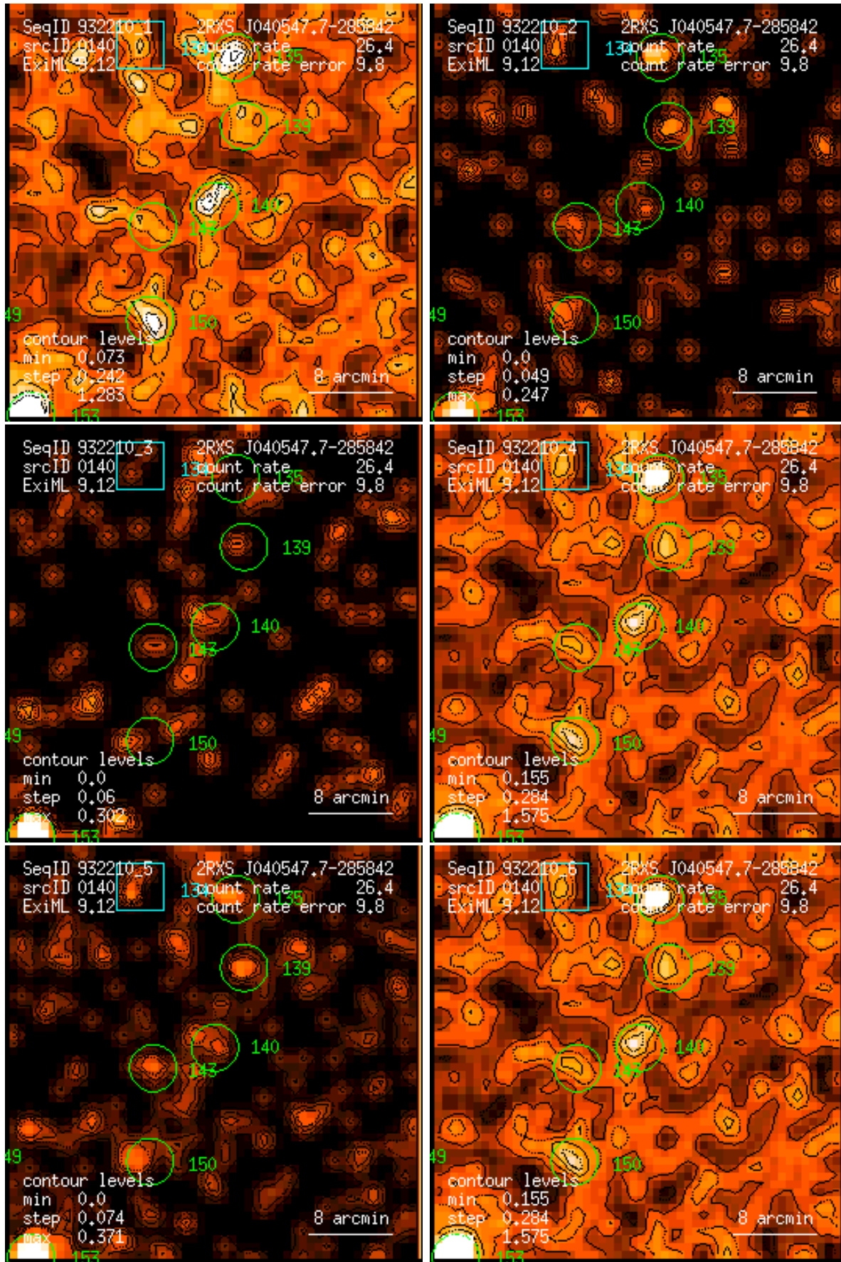
Figure 140: RASS 932210: detection 0140: band rate images, Gaussian filter: (1) PSPC channels 11 – 41, (2) 52 – 90, (3) 91 – 201, (4) 11 – 235, (5) 52 – 201, (6) 11 – 201. Broad band rates in counts/ks. Band rate contour levels in counts/ks/arcmin 2 .
