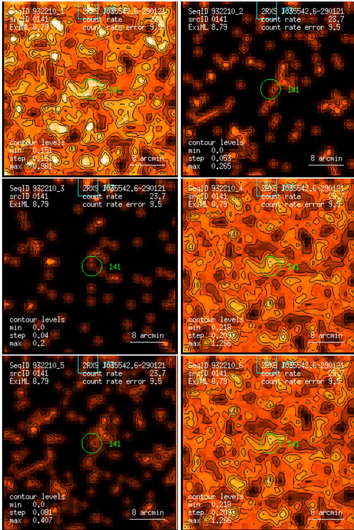
Figure 141: RASS 932210: detection 0141: band rate images, Gaussian filter: (1) PSPC channels 11 – 41, (2) 52 – 90, (3) 91 – 201, (4) 11 – 235, (5) 52 – 201, (6) 11 – 201. Broad band rates in counts/ks. Band rate contour levels in counts/ks/arcmin 2 .
