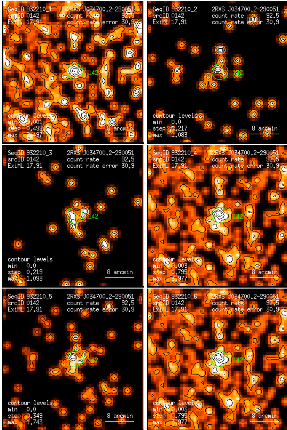
Figure 142: RASS 932210: detection 0142: band rate images, Gaussian filter: (1) PSPC channels 11 – 41, (2) 52 – 90, (3) 91 – 201, (4) 11 – 235, (5) 52 – 201, (6) 11 – 201. Broad band rates in counts/ks. Band rate contour levels in counts/ks/arcmin 2 .
