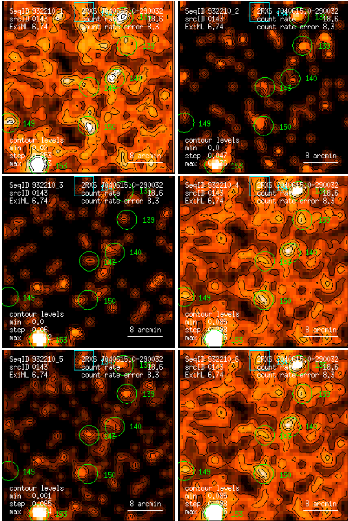
Figure 143: RASS 932210: detection 0143: band rate images, Gaussian filter: (1) PSPC channels 11 – 41, (2) 52 – 90, (3) 91 – 201, (4) 11 – 235, (5) 52 – 201, (6) 11 – 201. Broad band rates in counts/ks. Band rate contour levels in counts/ks/arcmin 2 .
