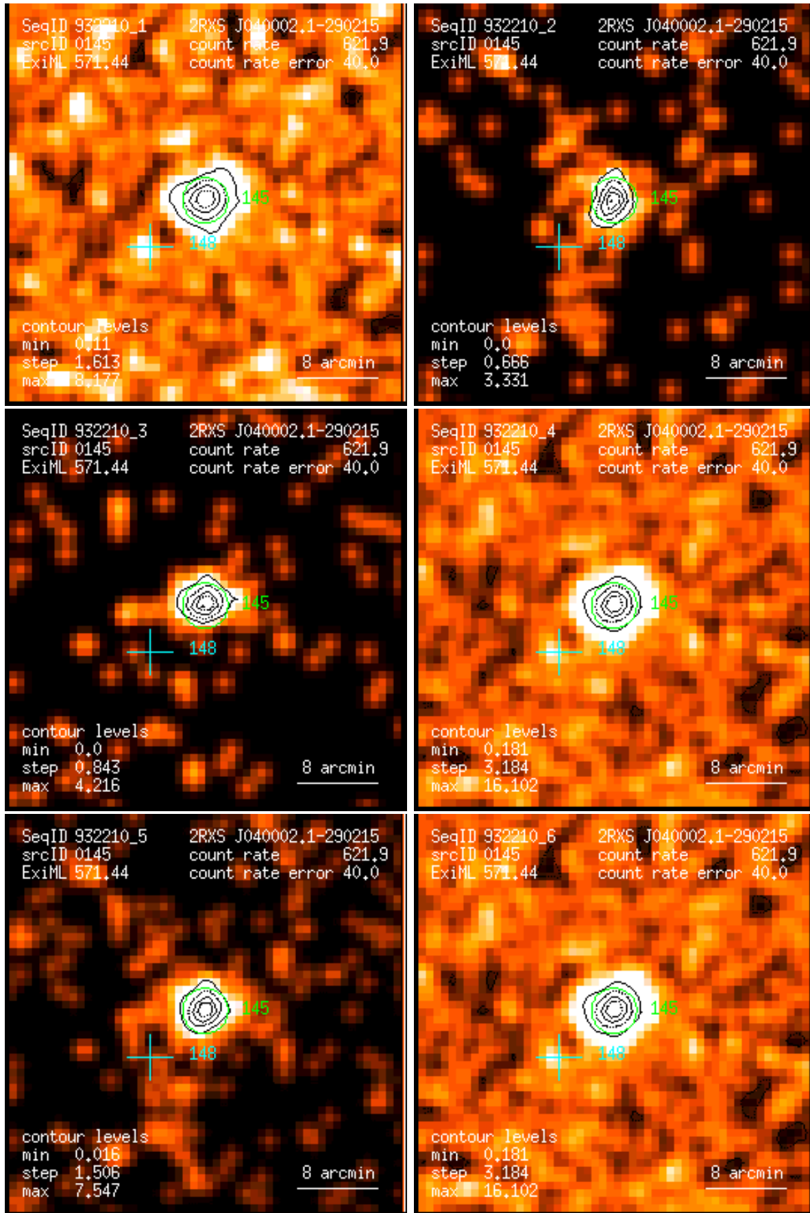
Figure 145: RASS 932210: detection 0145: band rate images, Gaussian filter: (1) PSPC channels 11 – 41, (2) 52 – 90, (3) 91 – 201, (4) 11 – 235, (5) 52 – 201, (6) 11 – 201. Broad band rates in counts/ks. Band rate contour levels in counts/ks/arcmin 2 .
