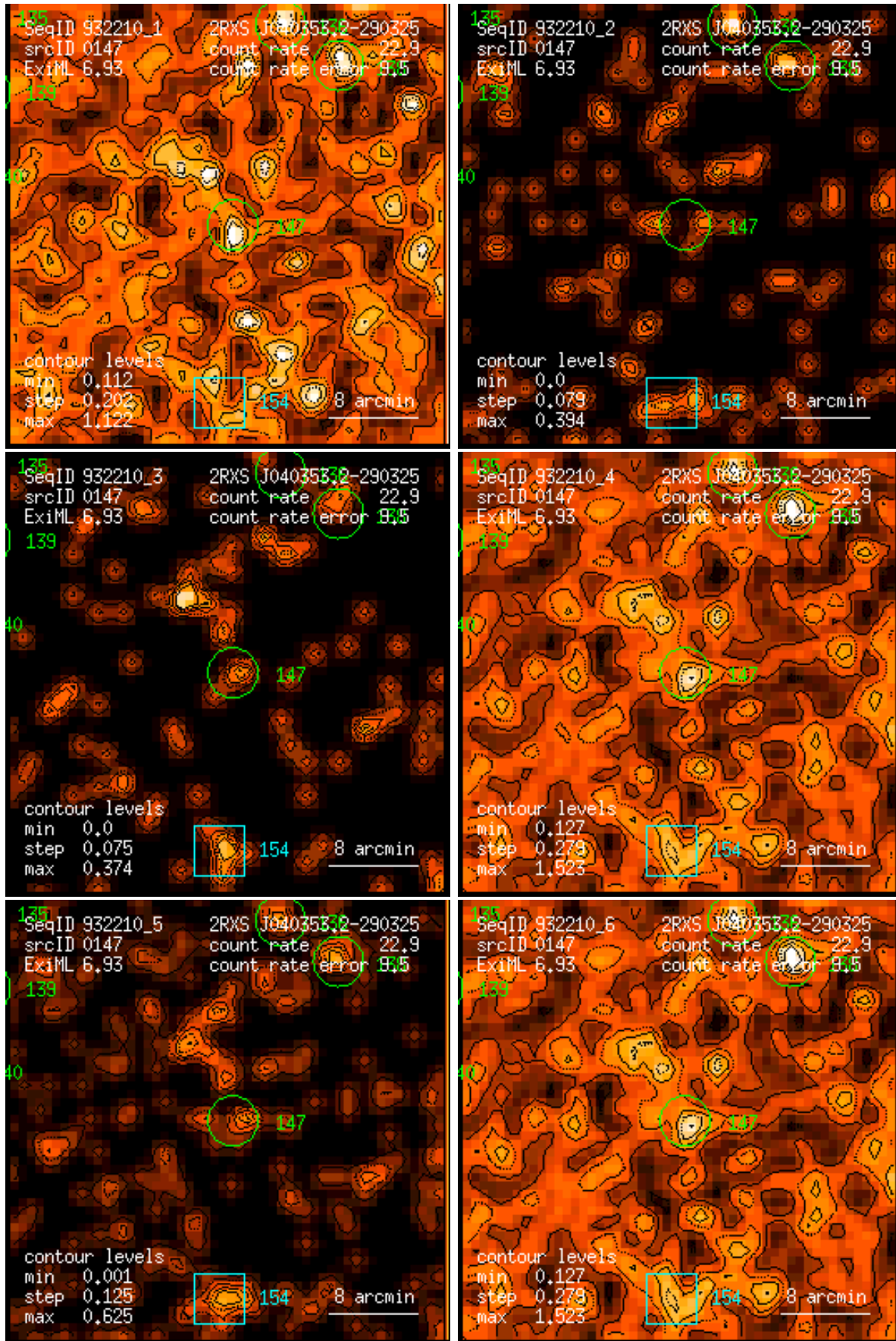
Figure 147: RASS 932210: detection 0147: band rate images, Gaussian filter: (1) PSPC channels 11 – 41, (2) 52 – 90, (3) 91 – 201, (4) 11 – 235, (5) 52 – 201, (6) 11 – 201. Broad band rates in counts/ks. Band rate contour levels in counts/ks/arcmin 2 .
