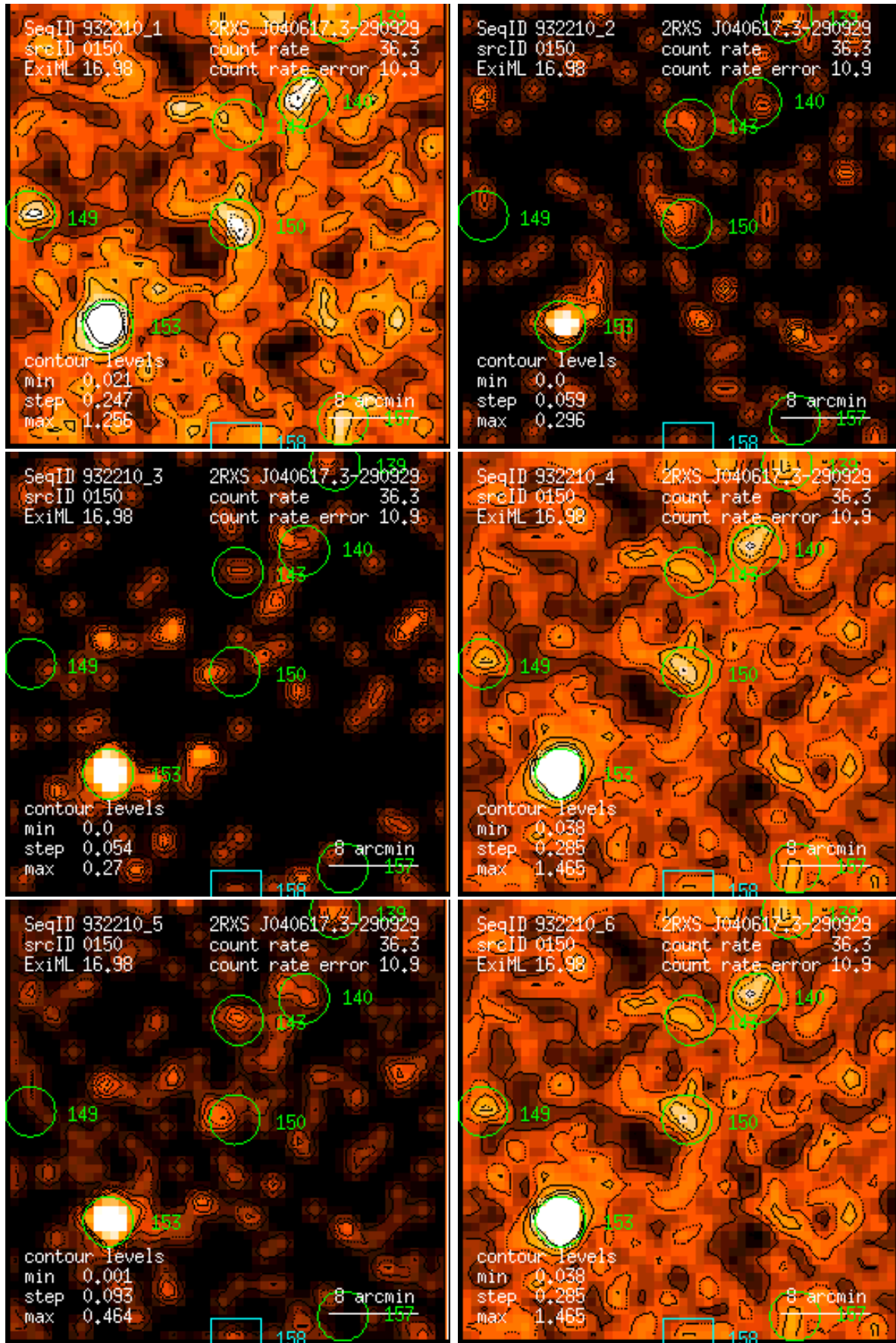
Figure 150: RASS 932210: detection 0150: band rate images, Gaussian filter: (1) PSPC channels 11 – 41, (2) 52 – 90, (3) 91 – 201, (4) 11 – 235, (5) 52 – 201, (6) 11 – 201. Broad band rates in counts/ks. Band rate contour levels in counts/ks/arcmin 2 .
