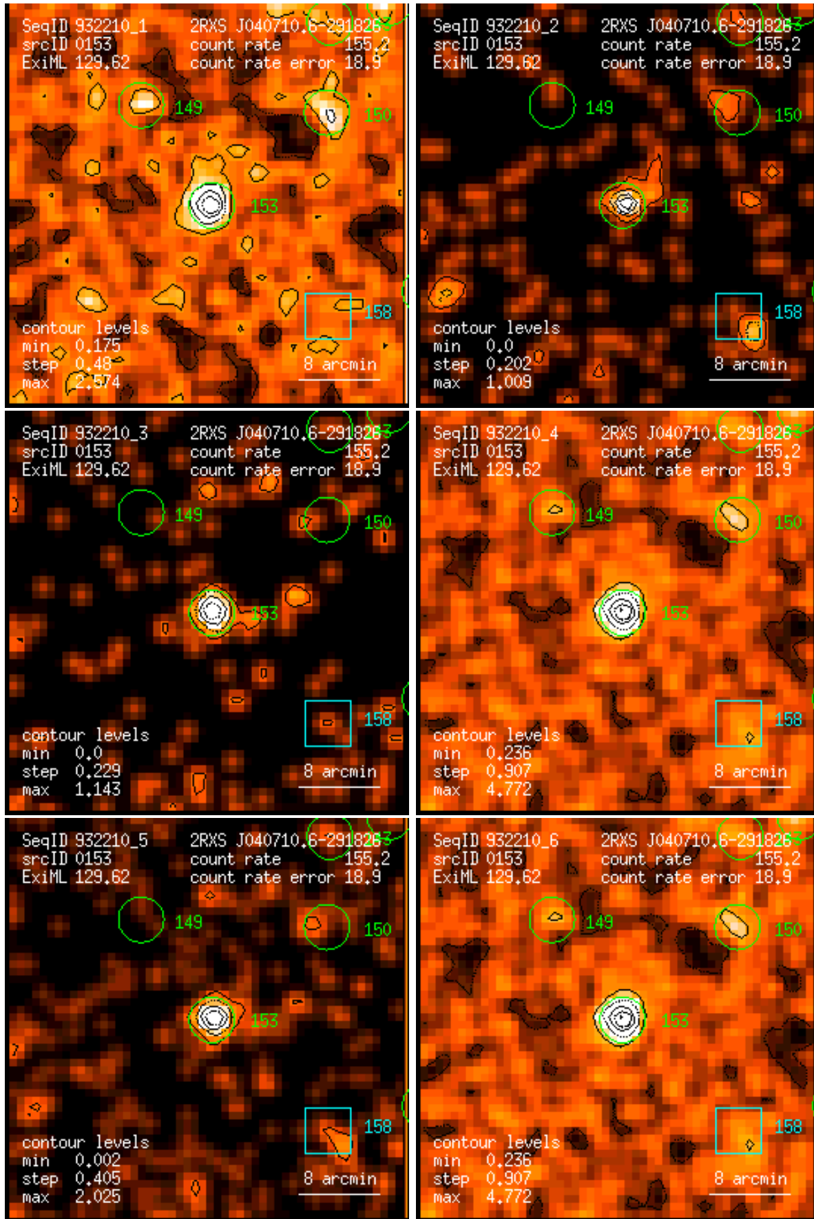
Figure 153: RASS 932210: detection 0153: band rate images, Gaussian filter: (1) PSPC channels 11 – 41, (2) 52 – 90, (3) 91 – 201, (4) 11 – 235, (5) 52 – 201, (6) 11 – 201. Broad band rates in counts/ks. Band rate contour levels in counts/ks/arcmin 2 .
