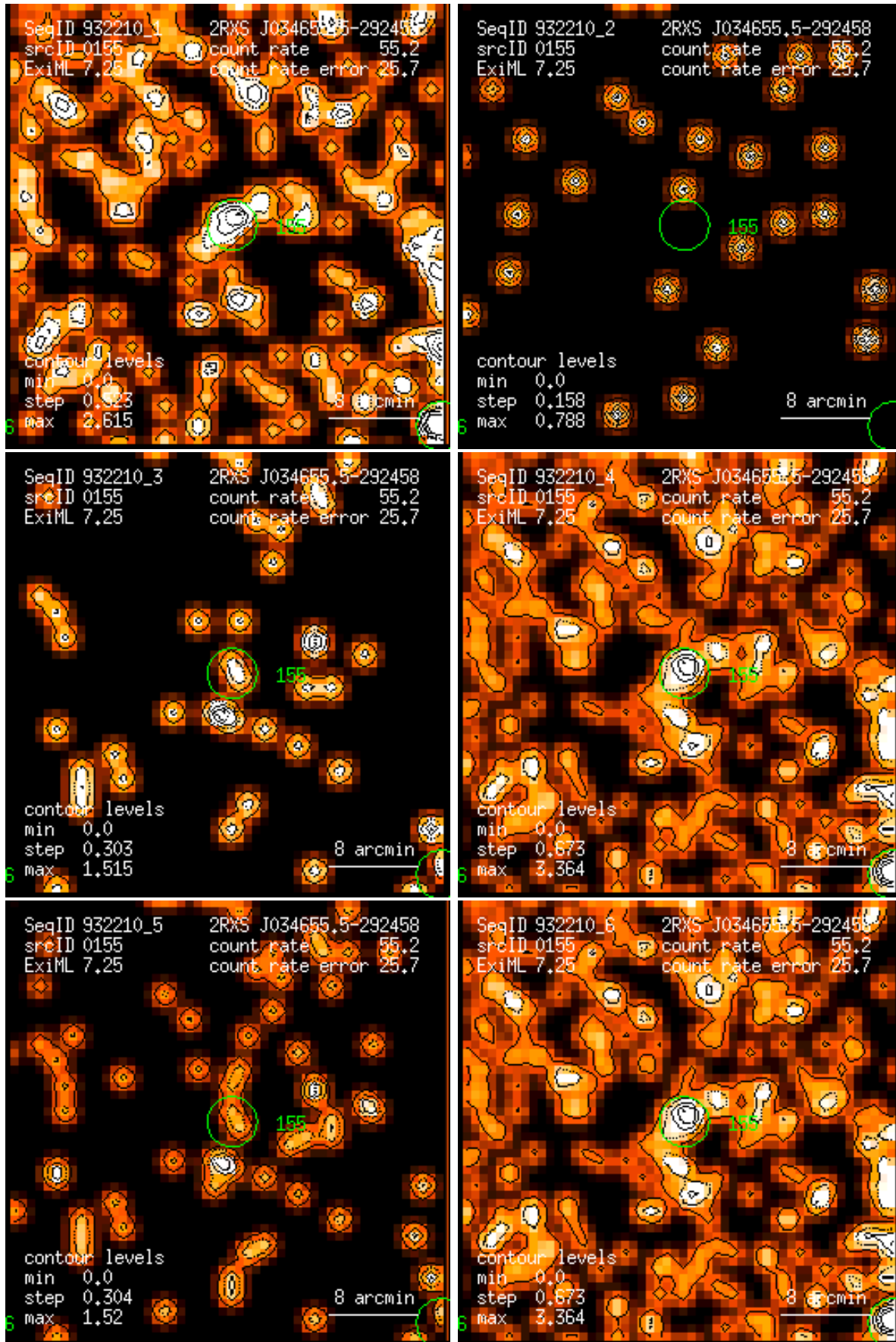
Figure 155: RASS 932210: detection 0155: band rate images, Gaussian filter: (1) PSPC channels 11 – 41, (2) 52 – 90, (3) 91 – 201, (4) 11 – 235, (5) 52 – 201, (6) 11 – 201. Broad band rates in counts/ks. Band rate contour levels in counts/ks/arcmin 2 .
