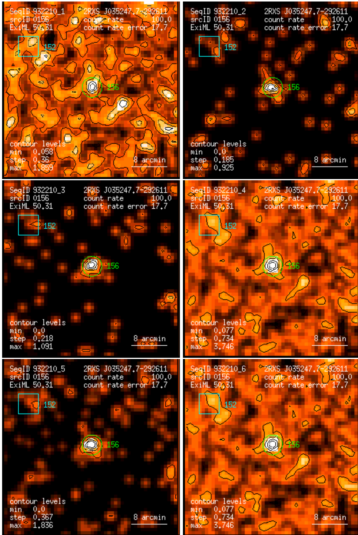
Figure 156: RASS 932210: detection 0156: band rate images, Gaussian filter: (1) PSPC channels 11 – 41, (2) 52 – 90, (3) 91 – 201, (4) 11 – 235, (5) 52 – 201, (6) 11 – 201. Broad band rates in counts/ks. Band rate contour levels in counts/ks/arcmin 2 .
