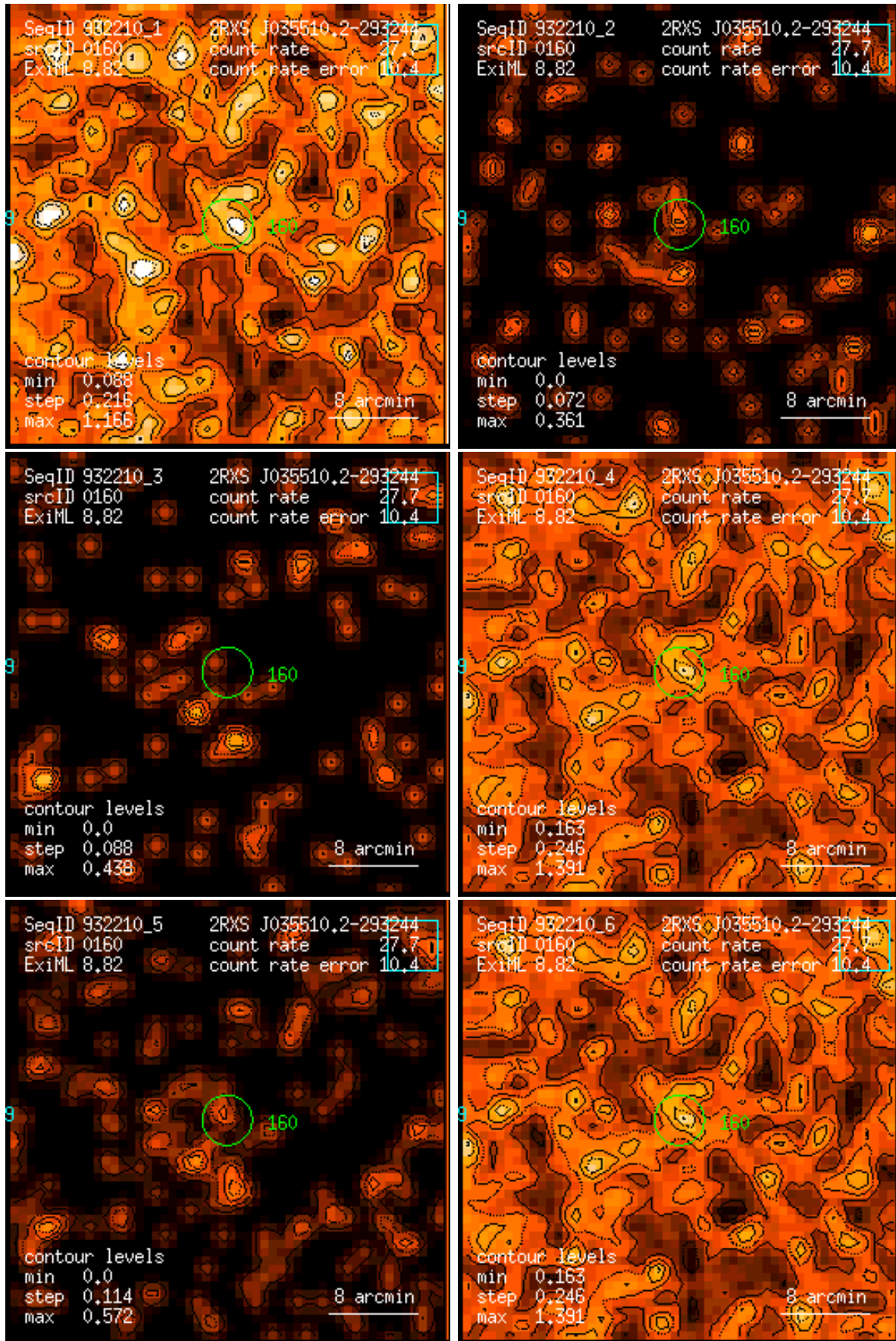
Figure 160: RASS 932210: detection 0160: band rate images, Gaussian filter: (1) PSPC channels 11 – 41, (2) 52 – 90, (3) 91 – 201, (4) 11 – 235, (5) 52 – 201, (6) 11 – 201. Broad band rates in counts/ks. Band rate contour levels in counts/ks/arcmin 2 .
