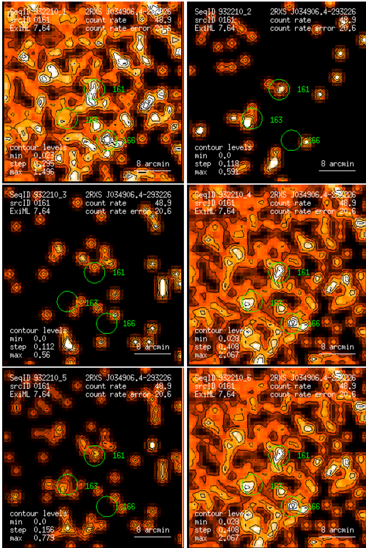
Figure 161: RASS 932210: detection 0161: band rate images, Gaussian filter: (1) PSPC channels 11 – 41, (2) 52 – 90, (3) 91 – 201, (4) 11 – 235, (5) 52 – 201, (6) 11 – 201. Broad band rates in counts/ks. Band rate contour levels in counts/ks/arcmin 2 .
