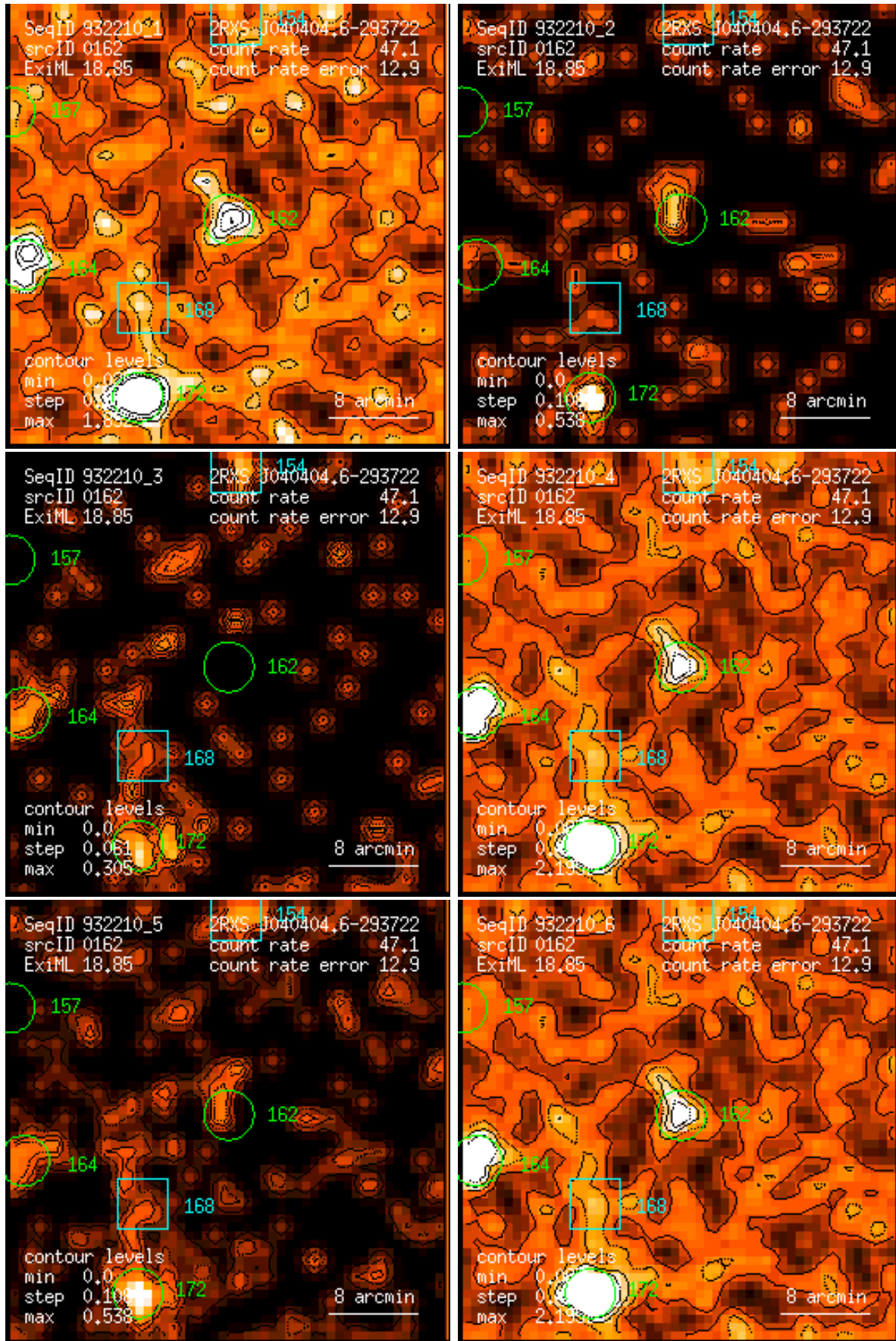
Figure 162: RASS 932210: detection 0162: band rate images, Gaussian filter: (1) PSPC channels 11 – 41, (2) 52 – 90, (3) 91 – 201, (4) 11 – 235, (5) 52 – 201, (6) 11 – 201. Broad band rates in counts/ks. Band rate contour levels in counts/ks/arcmin 2 .
