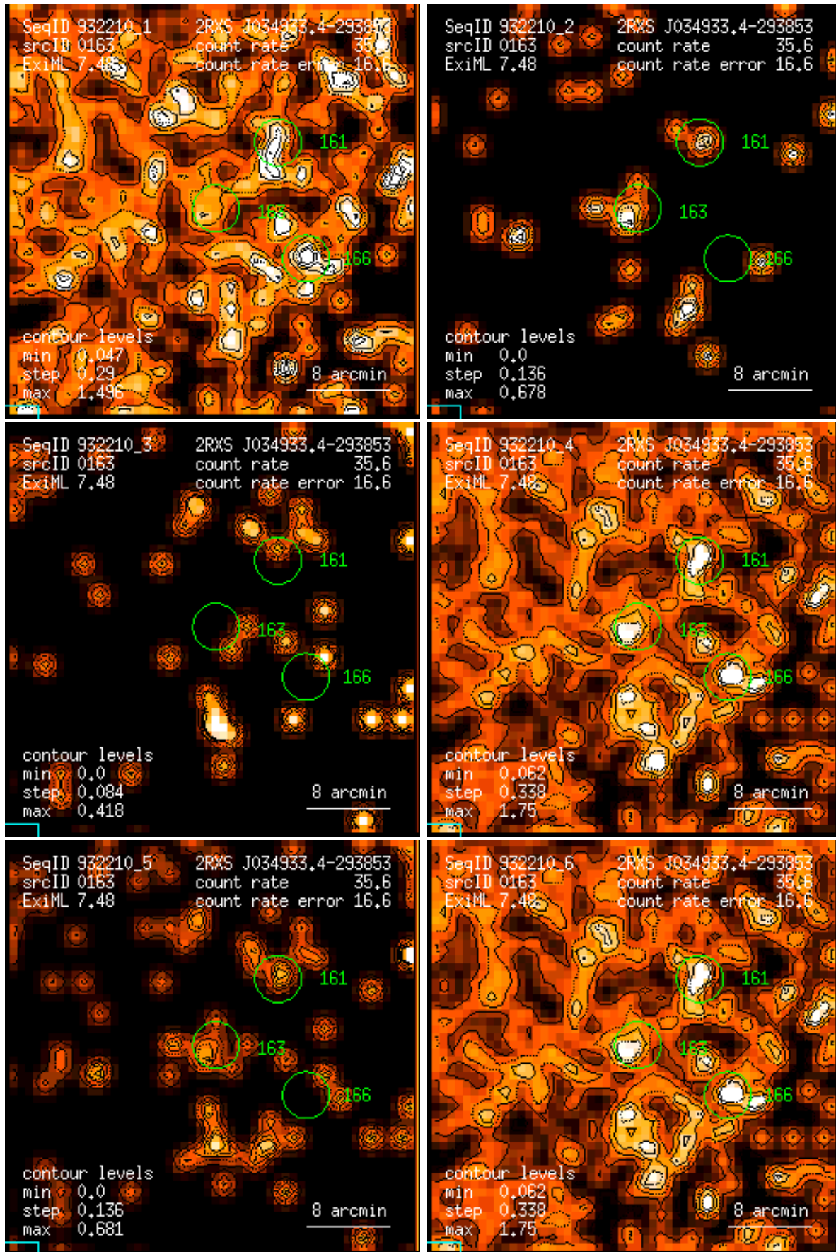
Figure 163: RASS 932210: detection 0163: band rate images, Gaussian filter: (1) PSPC channels 11 – 41, (2) 52 – 90, (3) 91 – 201, (4) 11 – 235, (5) 52 – 201, (6) 11 – 201. Broad band rates in counts/ks. Band rate contour levels in counts/ks/arcmin 2 .
