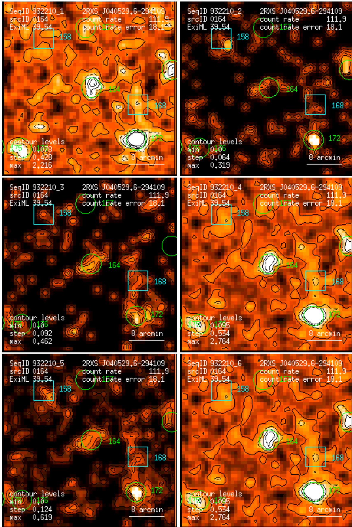
Figure 164: RASS 932210: detection 0164: band rate images, Gaussian filter: (1) PSPC channels 11 – 41, (2) 52 – 90, (3) 91 – 201, (4) 11 – 235, (5) 52 – 201, (6) 11 – 201. Broad band rates in counts/ks. Band rate contour levels in counts/ks/arcmin 2 .
