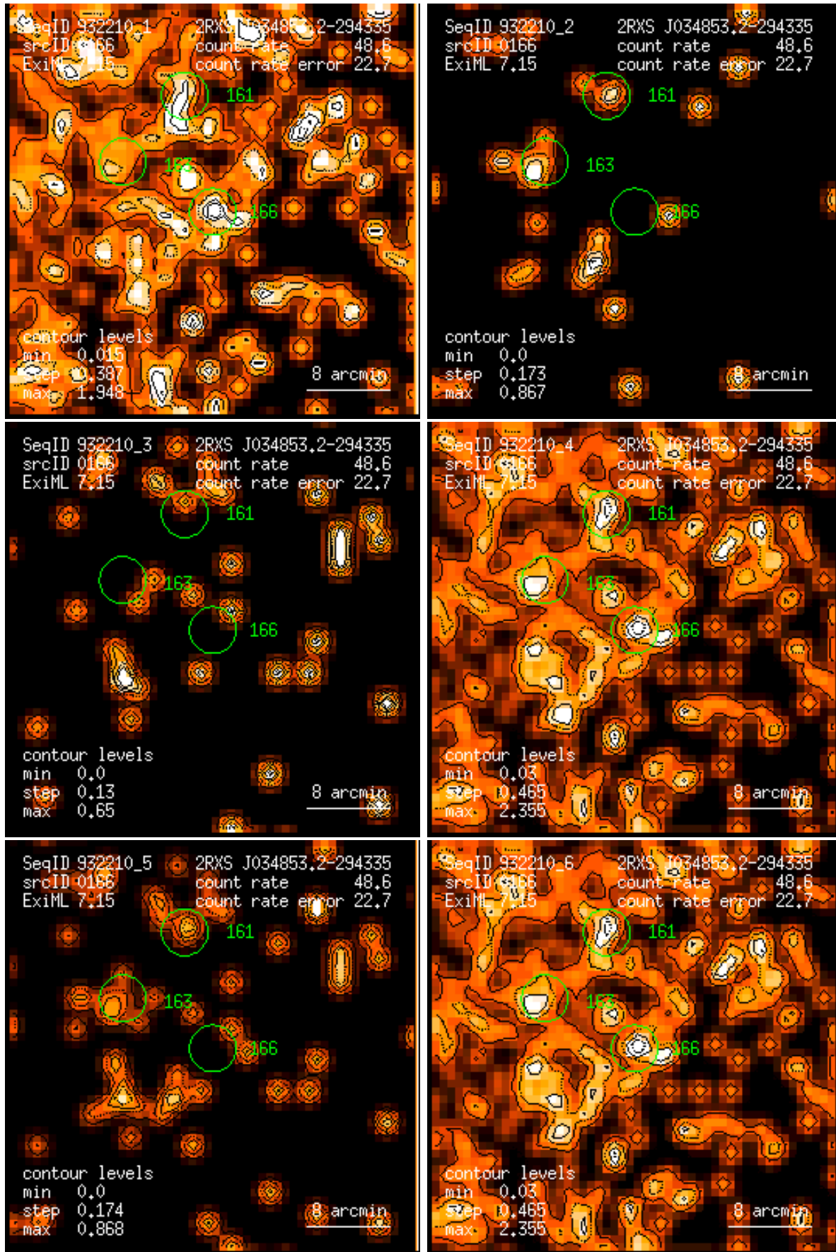
Figure 166: RASS 932210: detection 0166: band rate images, Gaussian filter: (1) PSPC channels 11 – 41, (2) 52 – 90, (3) 91 – 201, (4) 11 – 235, (5) 52 – 201, (6) 11 – 201. Broad band rates in counts/ks. Band rate contour levels in counts/ks/arcmin 2 .
