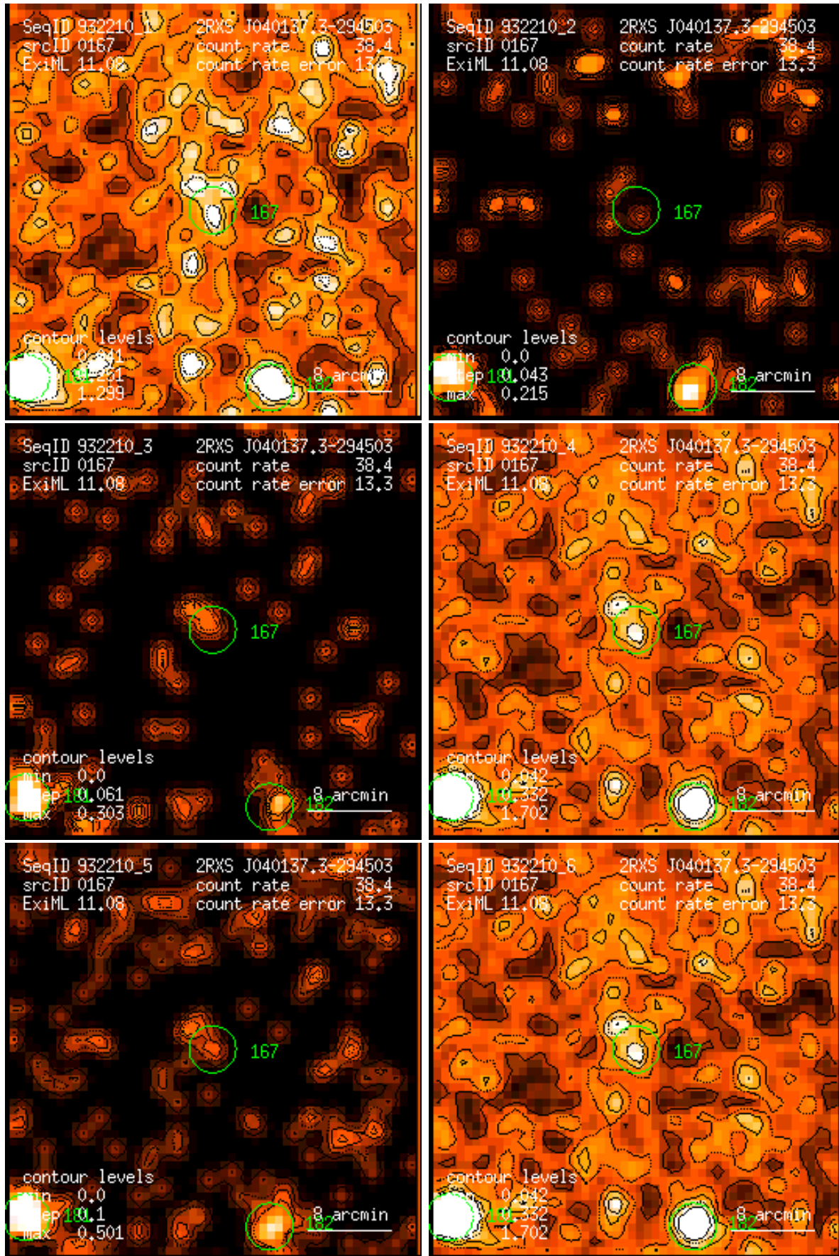
Figure 167: RASS 932210: detection 0167: band rate images, Gaussian filter: (1) PSPC channels 11 – 41, (2) 52 – 90, (3) 91 – 201, (4) 11 – 235, (5) 52 – 201, (6) 11 – 201. Broad band rates in counts/ks. Band rate contour levels in counts/ks/arcmin 2 .
