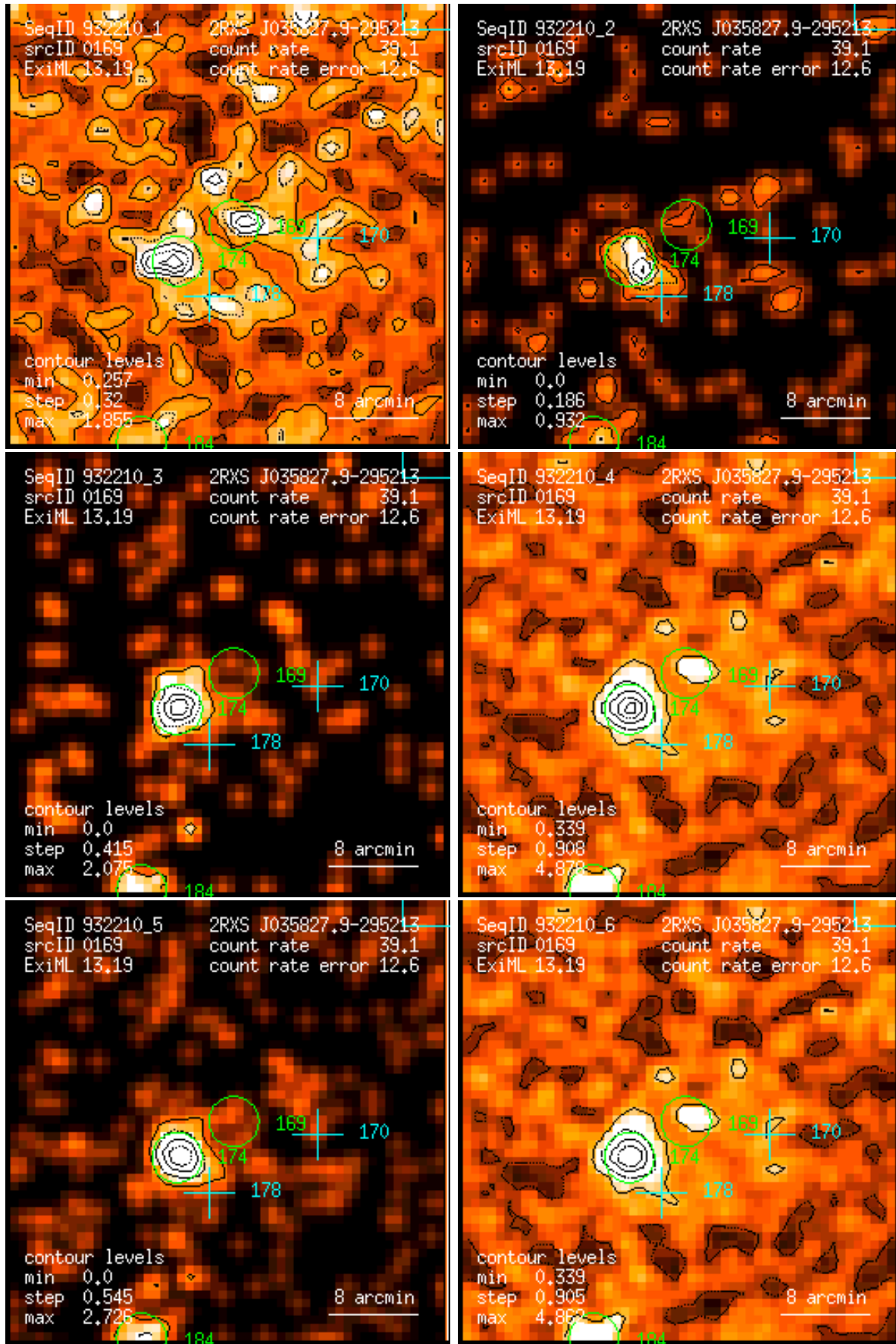
Figure 169: RASS 932210: detection 0169: band rate images, Gaussian filter: (1) PSPC channels 11 – 41, (2) 52 – 90, (3) 91 – 201, (4) 11 – 235, (5) 52 – 201, (6) 11 – 201. Broad band rates in counts/ks. Band rate contour levels in counts/ks/arcmin 2 .
