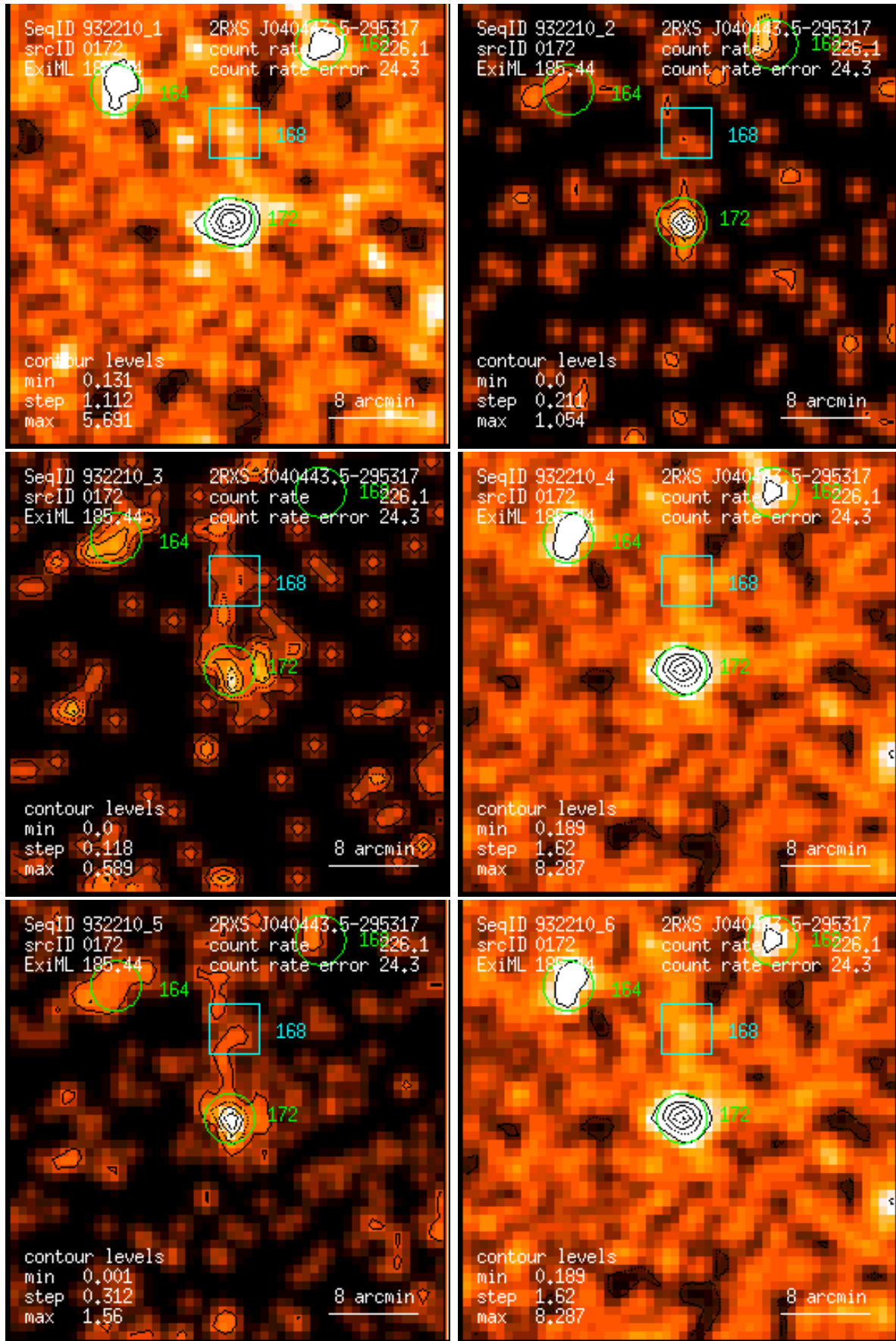
Figure 172: RASS 932210: detection 0172: band rate images, Gaussian filter: (1) PSPC channels 11 – 41, (2) 52 – 90, (3) 91 – 201, (4) 11 – 235, (5) 52 – 201, (6) 11 – 201. Broad band rates in counts/ks. Band rate contour levels in counts/ks/arcmin 2 .
