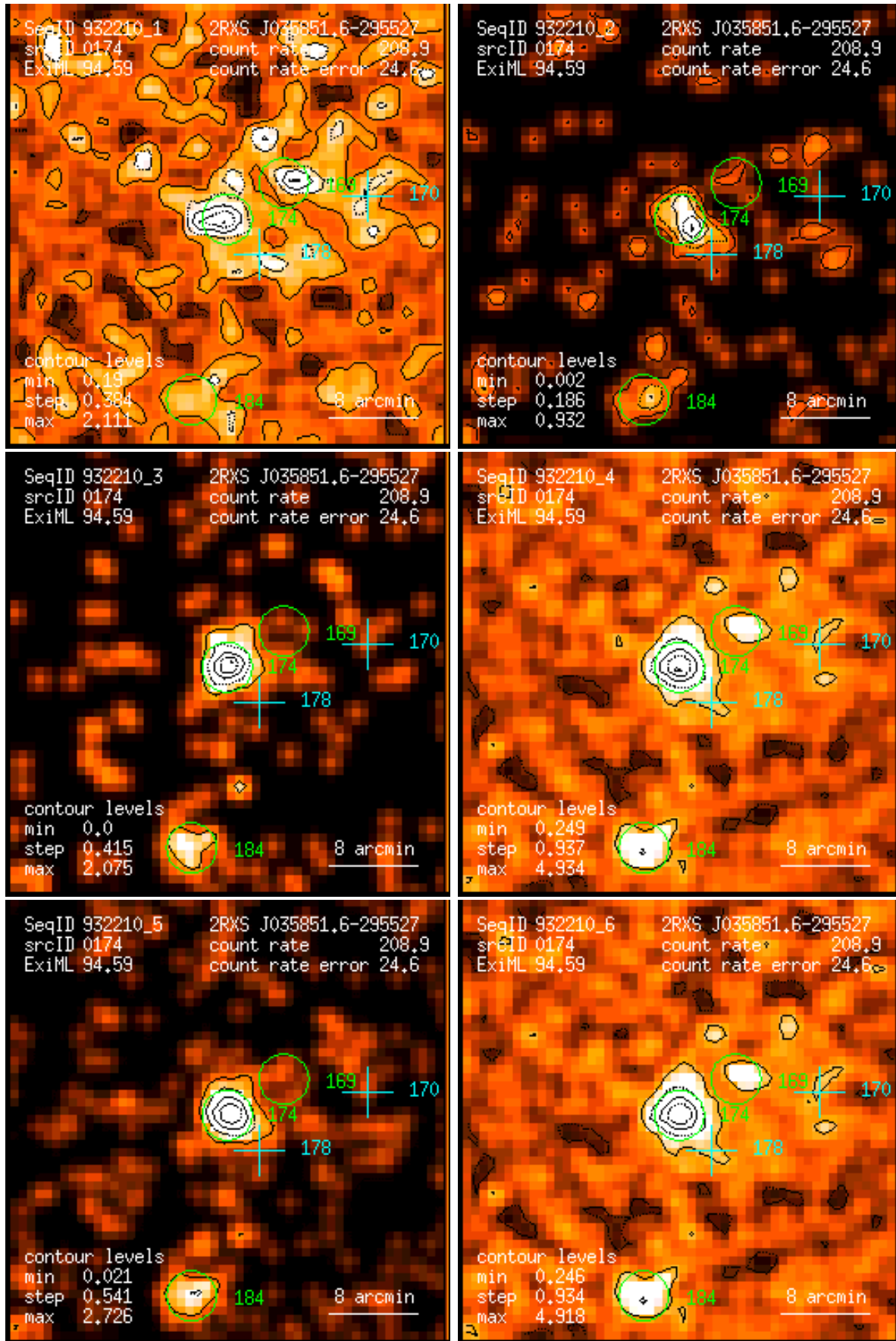
Figure 174: RASS 932210: detection 0174: band rate images, Gaussian filter: (1) PSPC channels 11 – 41, (2) 52 – 90, (3) 91 – 201, (4) 11 – 235, (5) 52 – 201, (6) 11 – 201. Broad band rates in counts/ks. Band rate contour levels in counts/ks/arcmin 2 .
