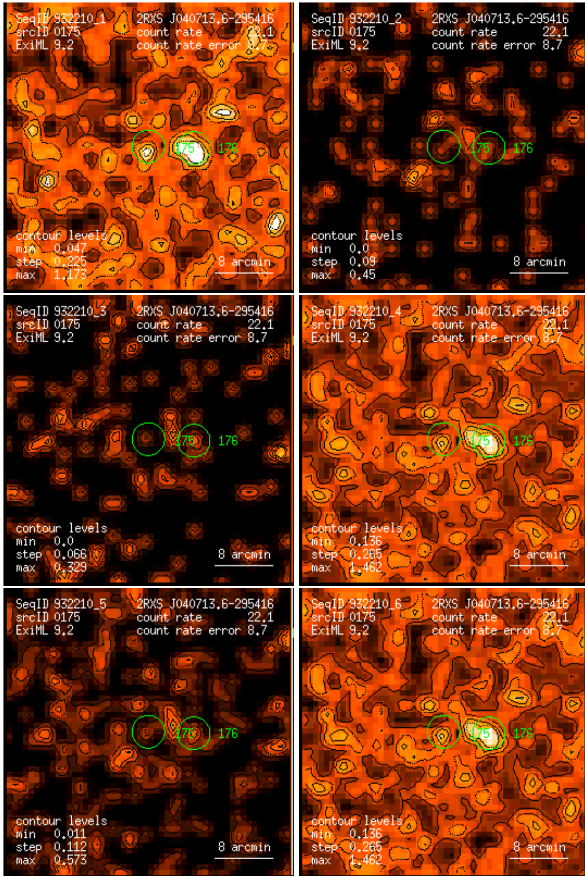
Figure 175: RASS 932210: detection 0175: band rate images, Gaussian filter: (1) PSPC channels 11 – 41, (2) 52 – 90, (3) 91 – 201, (4) 11 – 235, (5) 52 – 201, (6) 11 – 201. Broad band rates in counts/ks. Band rate contour levels in counts/ks/arcmin 2 .
