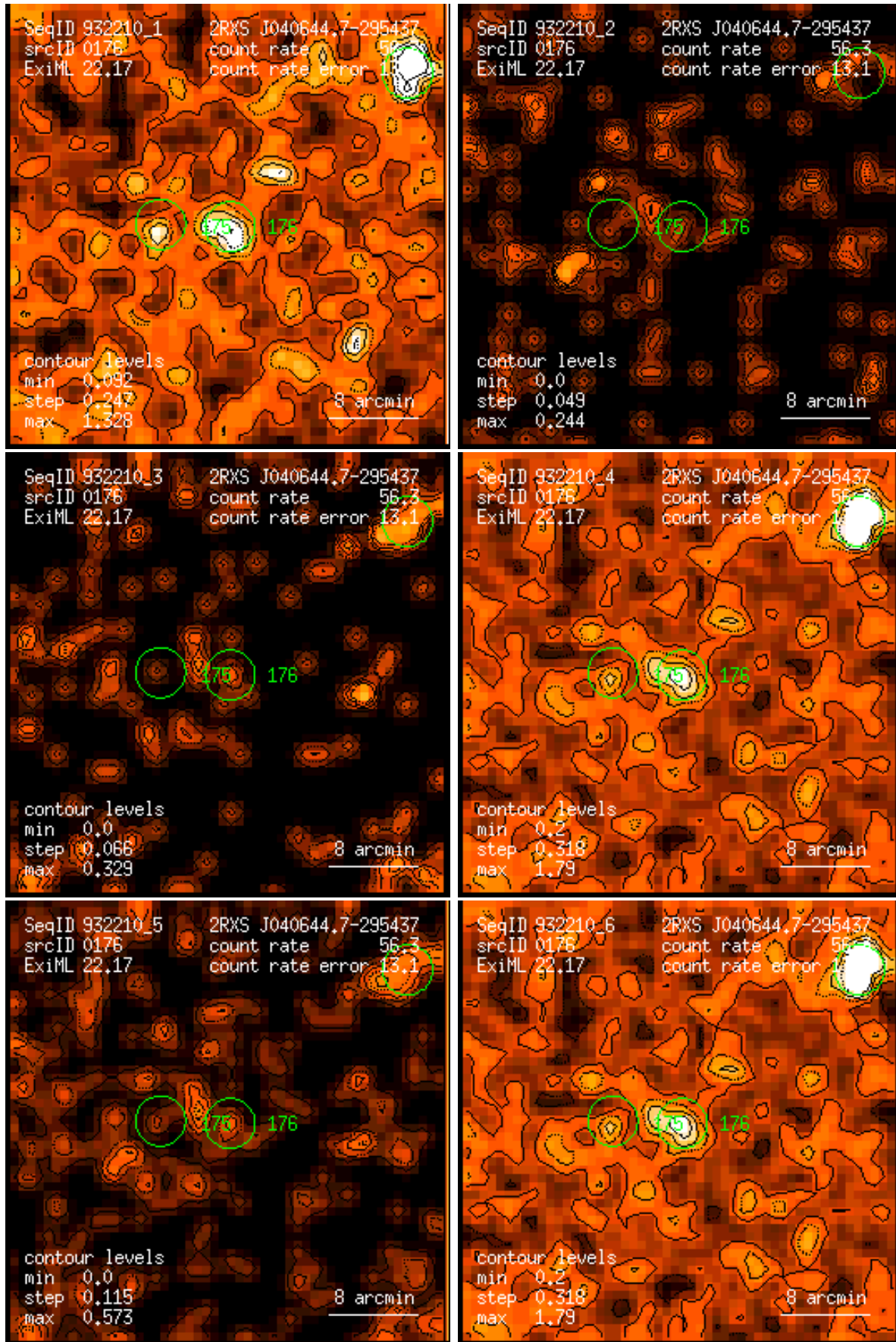
Figure 176: RASS 932210: detection 0176: band rate images, Gaussian filter: (1) PSPC channels 11 – 41, (2) 52 – 90, (3) 91 – 201, (4) 11 – 235, (5) 52 – 201, (6) 11 – 201. Broad band rates in counts/ks. Band rate contour levels in counts/ks/arcmin 2 .
