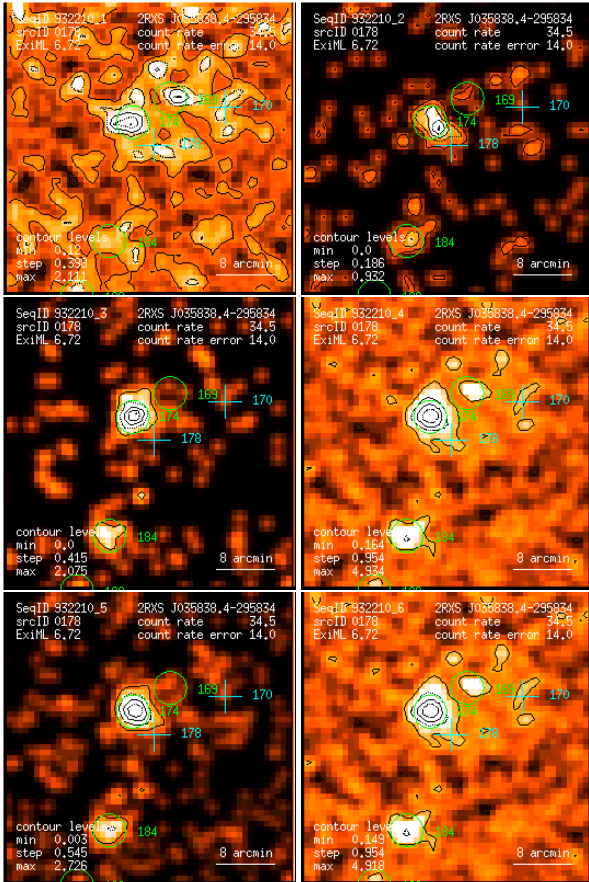
Figure 178: RASS 932210: detection 0178: band rate images, Gaussian filter: (1) PSPC channels 11 – 41, (2) 52 – 90, (3) 91 – 201, (4) 11 – 235, (5) 52 – 201, (6) 11 – 201. Broad band rates in counts/ks. Band rate contour levels in counts/ks/arcmin 2 .
