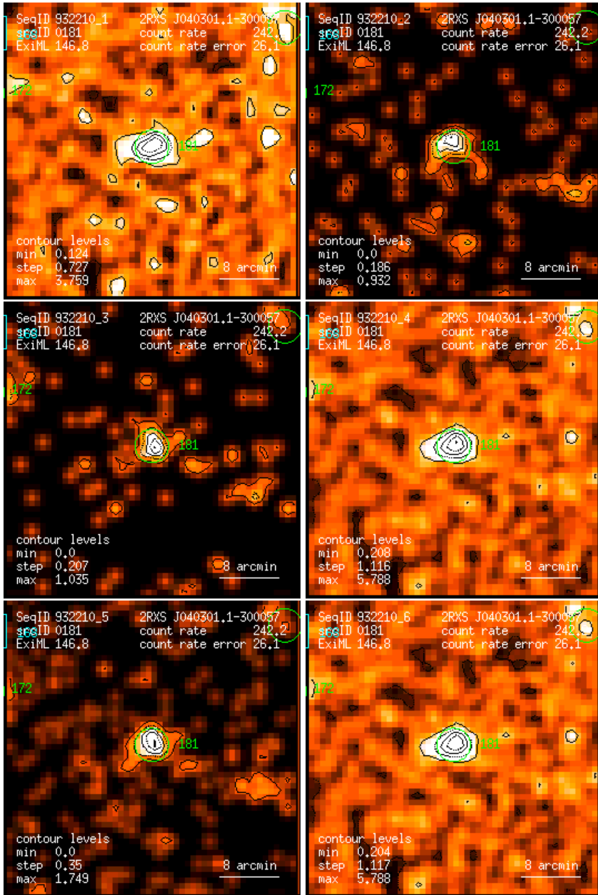
Figure 181: RASS 932210: detection 0181: band rate images, Gaussian filter: (1) PSPC channels 11 – 41, (2) 52 – 90, (3) 91 – 201, (4) 11 – 235, (5) 52 – 201, (6) 11 – 201. Broad band rates in counts/ks. Band rate contour levels in counts/ks/arcmin 2 .
