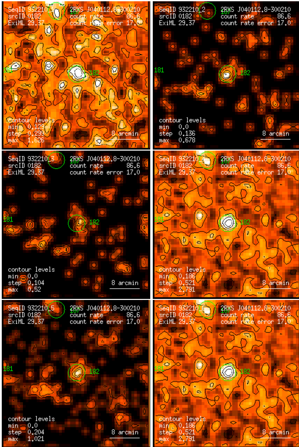
Figure 182: RASS 932210: detection 0182: band rate images, Gaussian filter: (1) PSPC channels 11 – 41, (2) 52 – 90, (3) 91 – 201, (4) 11 – 235, (5) 52 – 201, (6) 11 – 201. Broad band rates in counts/ks. Band rate contour levels in counts/ks/arcmin 2 .
