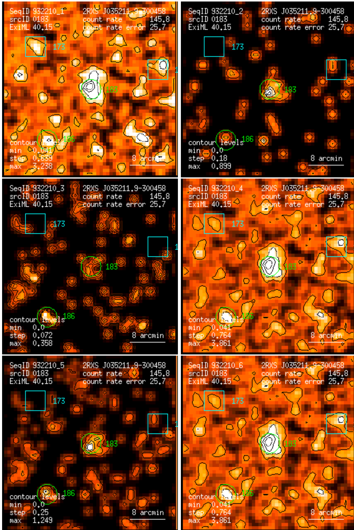
Figure 183: RASS 932210: detection 0183: band rate images, Gaussian filter: (1) PSPC channels 11 – 41, (2) 52 – 90, (3) 91 – 201, (4) 11 – 235, (5) 52 – 201, (6) 11 – 201. Broad band rates in counts/ks. Band rate contour levels in counts/ks/arcmin 2 .
