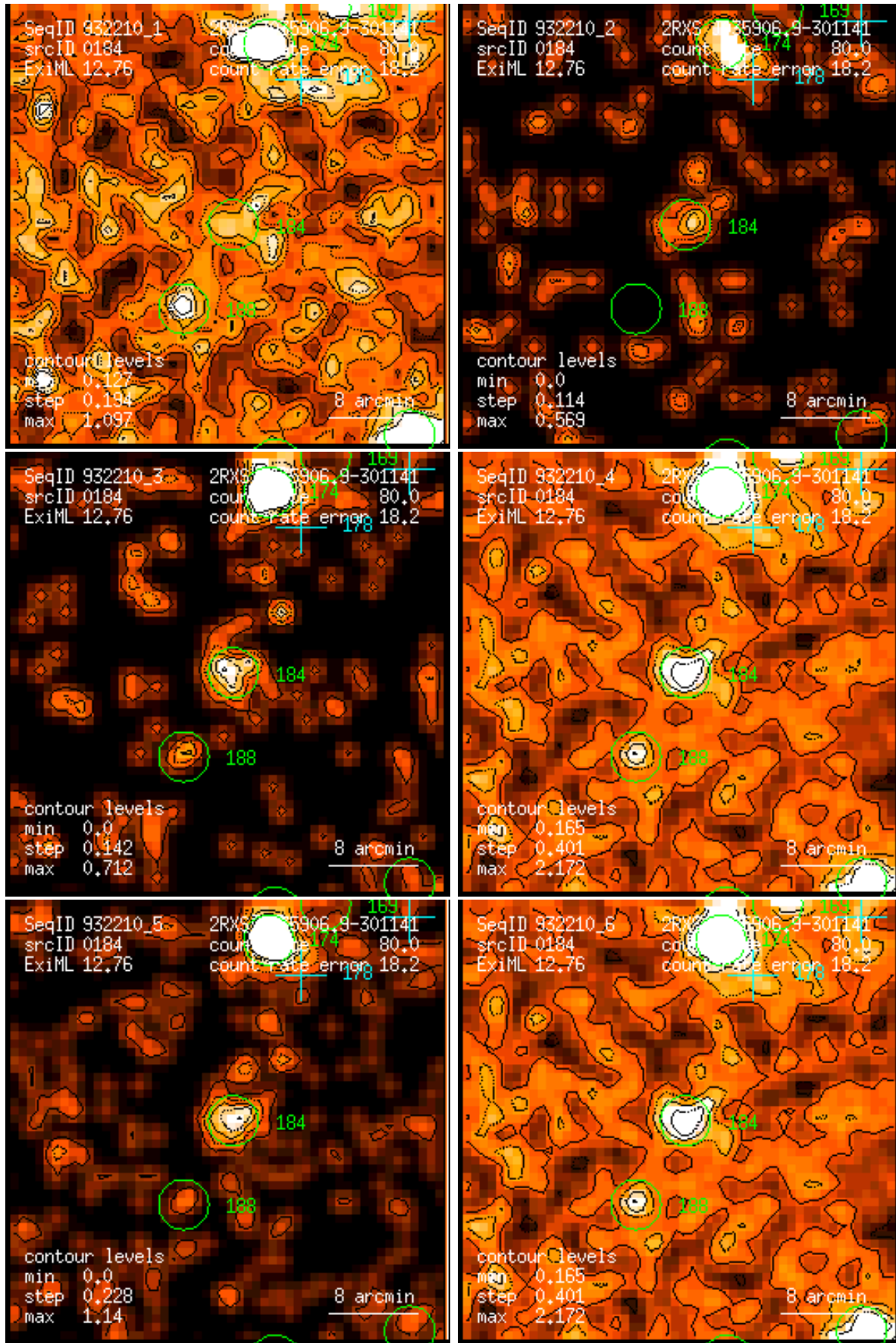
Figure 184: RASS 932210: detection 0184: band rate images, Gaussian filter: (1) PSPC channels 11 – 41, (2) 52 – 90, (3) 91 – 201, (4) 11 – 235, (5) 52 – 201, (6) 11 – 201. Broad band rates in counts/ks. Band rate contour levels in counts/ks/arcmin 2 .
